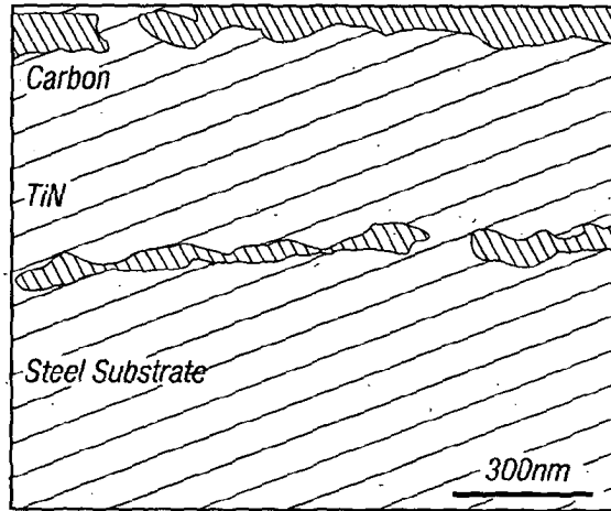
SEM cross section of TiN+C coating on 316L substrate
