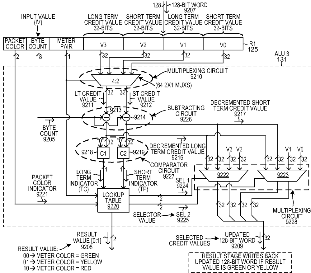
ATOMIC METERING COMMAND LOOKUP STAGE
