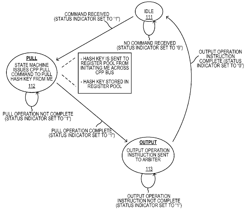
STATE MACHINE STATE DIAGRAM FIG. 16
