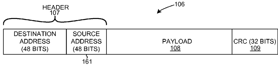
ETHERNET PACKET FIG. 15
