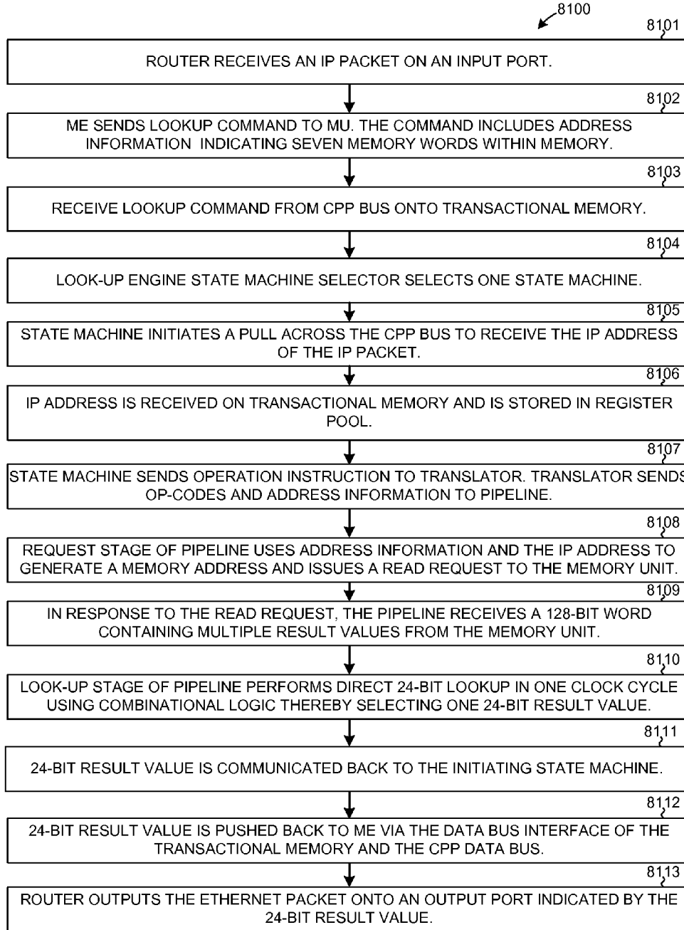
DIRECT 24-BIT LOOK-UP FLOWCHART FIG. 50
