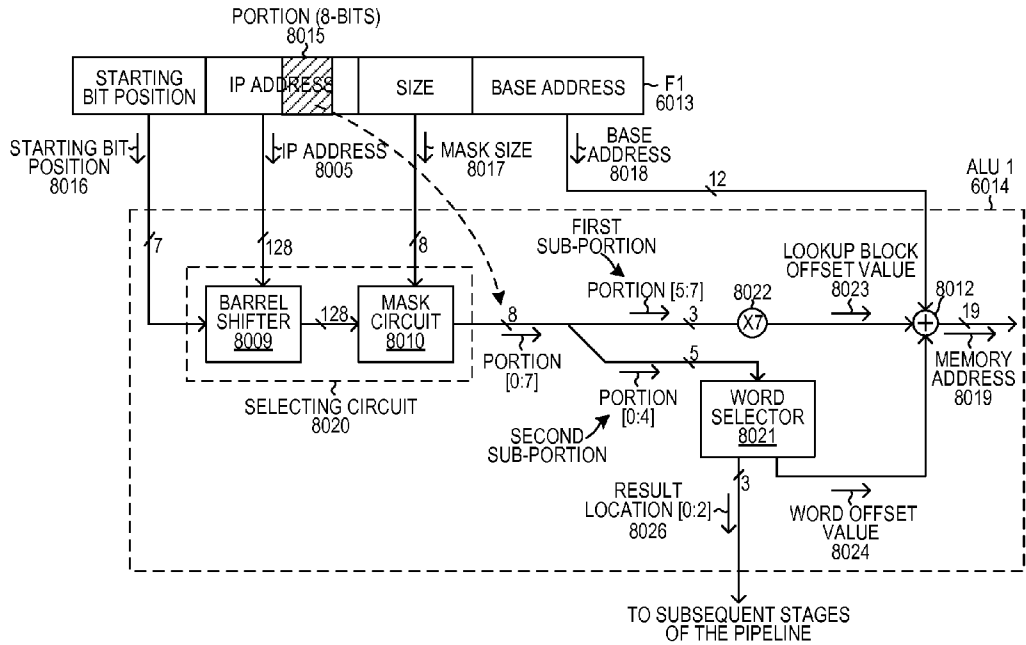
DIRECT 24-BIT REQUEST STAGE FIG. 48
