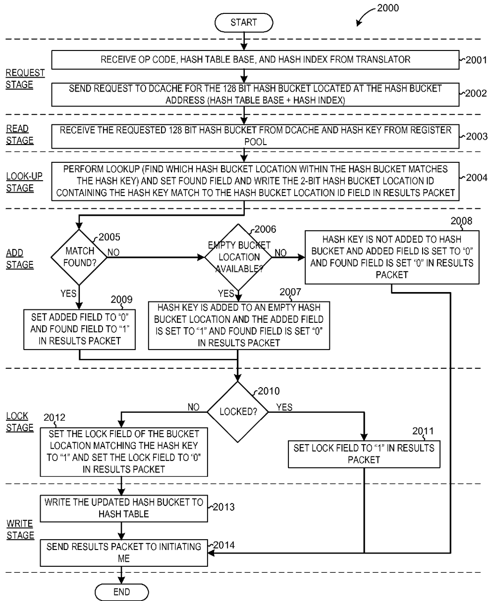
PIPELINE OPERATIONAL FLOW FIG. 24
