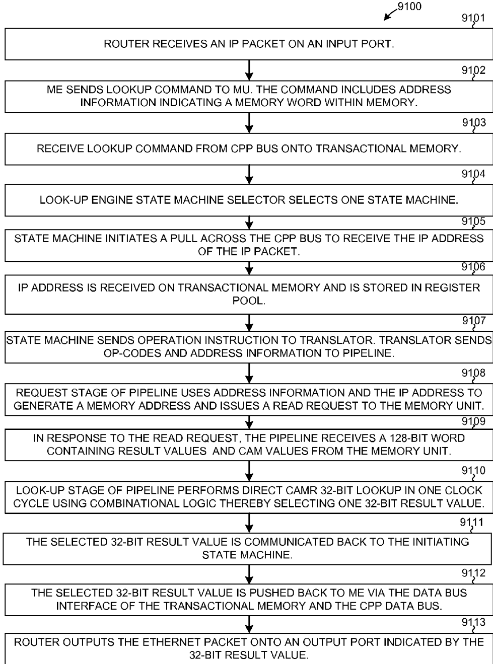
CAMR 32-BIT LOOKUP FLOWCHART FIG. 55
