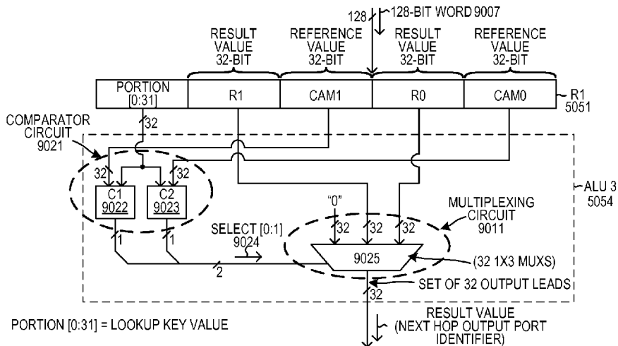
DIRECT CAMR 32-BIT LOOKUP STAGE
