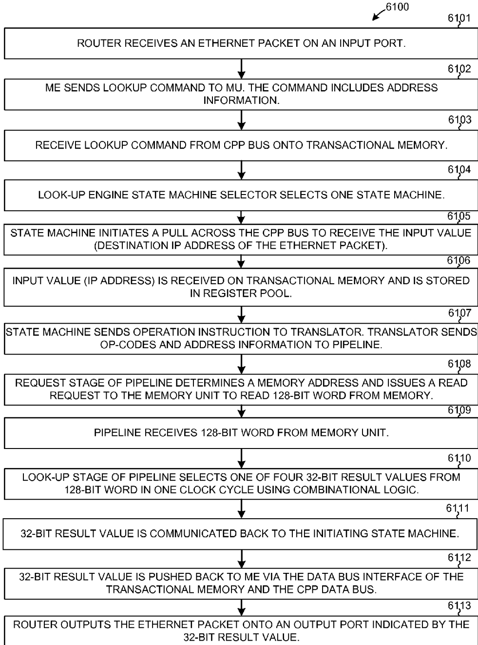
DIRECT 32-BIT LOOKUP FLOWCHART FIG. 44
