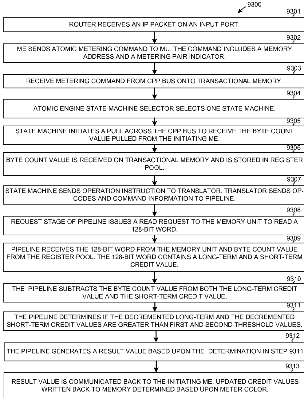
ATOMIC METERING COMMAND FLOWCHART FIG. 62
