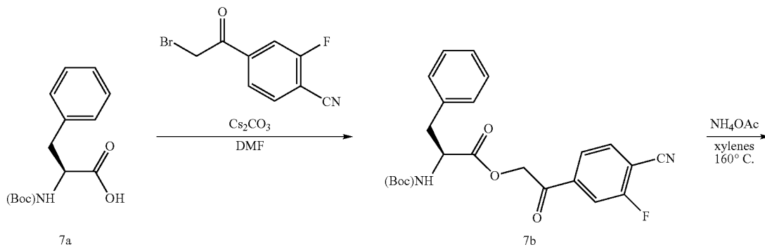
Scheme 7
