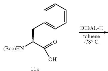
Scheme 11
