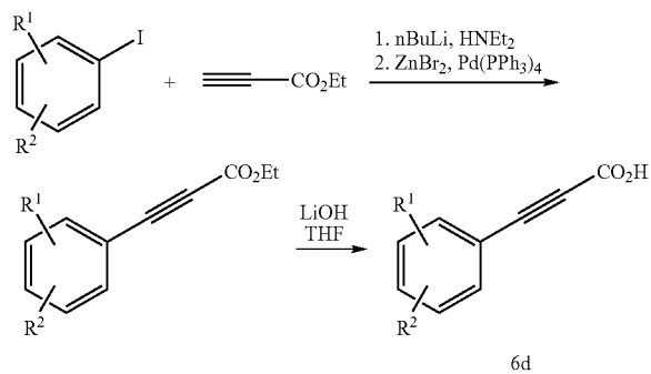
Scheme 6A
