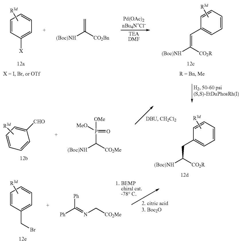
Scheme 12
