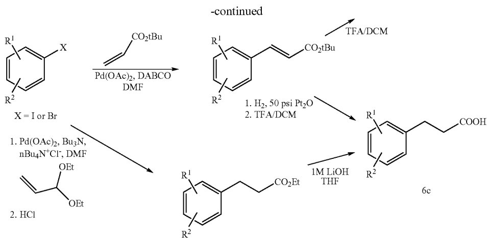
Scheme 6A
