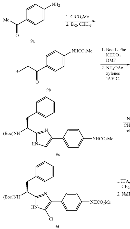
Scheme 9
