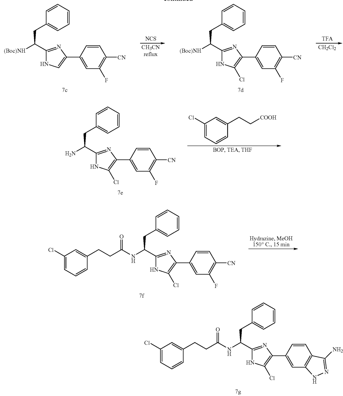
Scheme 8
