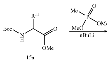
Scheme 15
