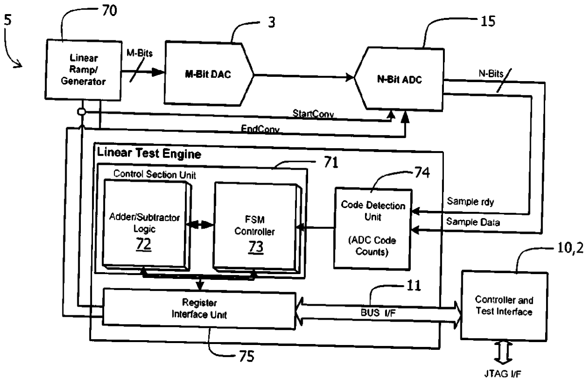
Fig. 6: Linear Test Engine
