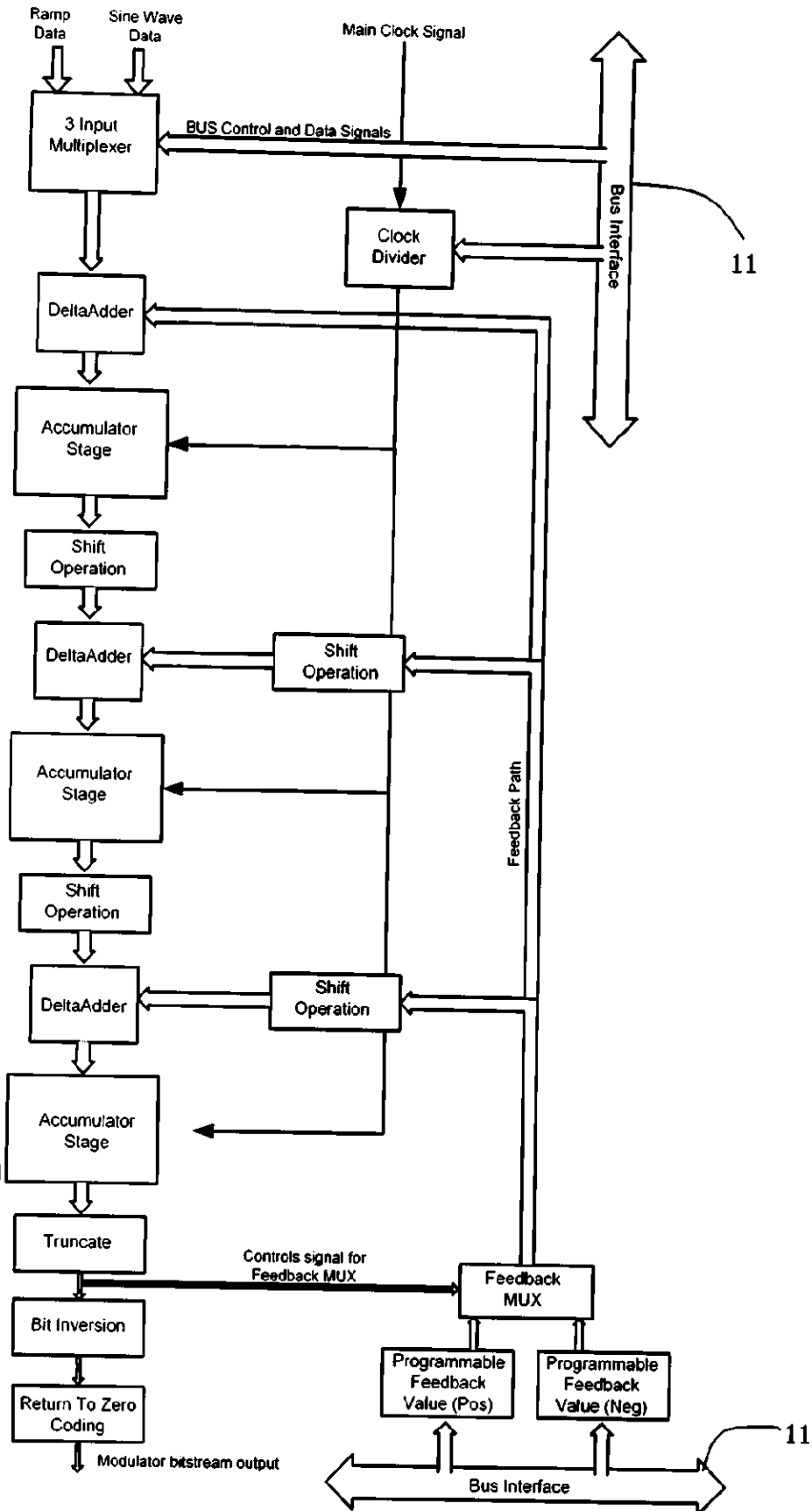
Fig. 3: Programmable DAC Architecture
