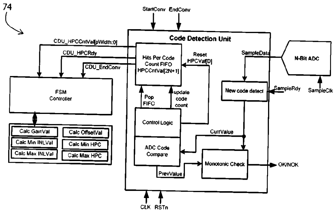
Fig. 7: Linear Test Engine - Code Detection Unit
