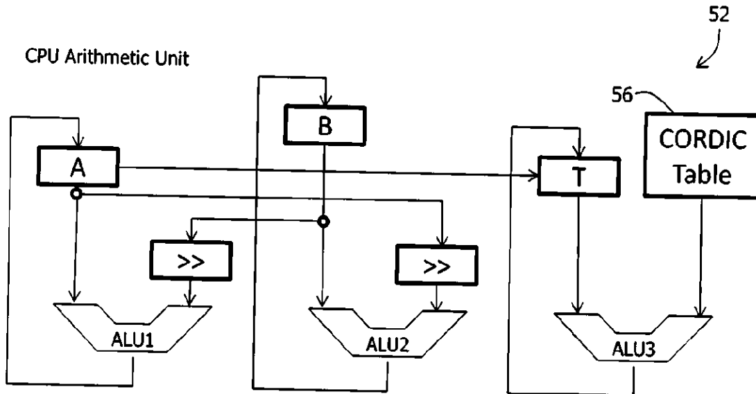
Fig. 5: Dynamic Test Engine - Arithmetic Unit
