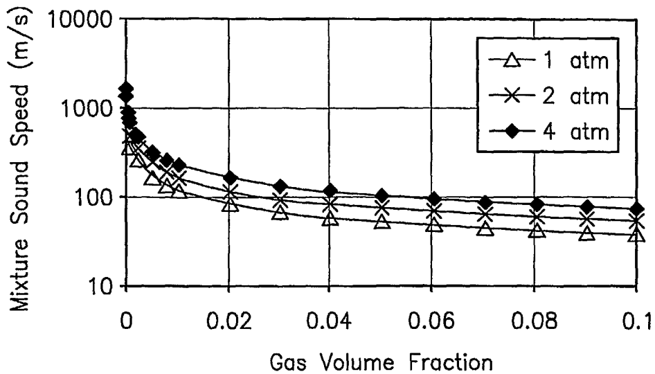
SOS as Function of Entrained Air (5% consistency)
