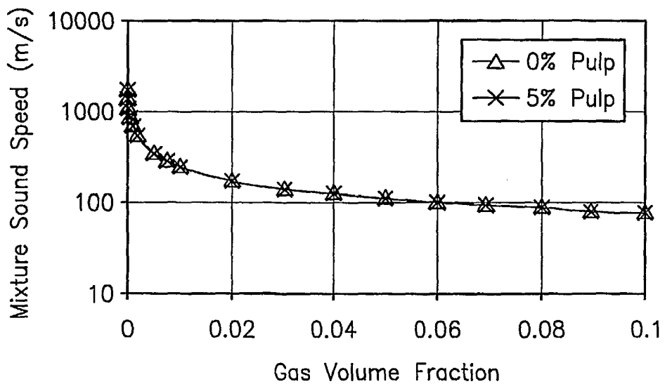
SOS as Function of Entrained Air ( \rho=4 atm)
