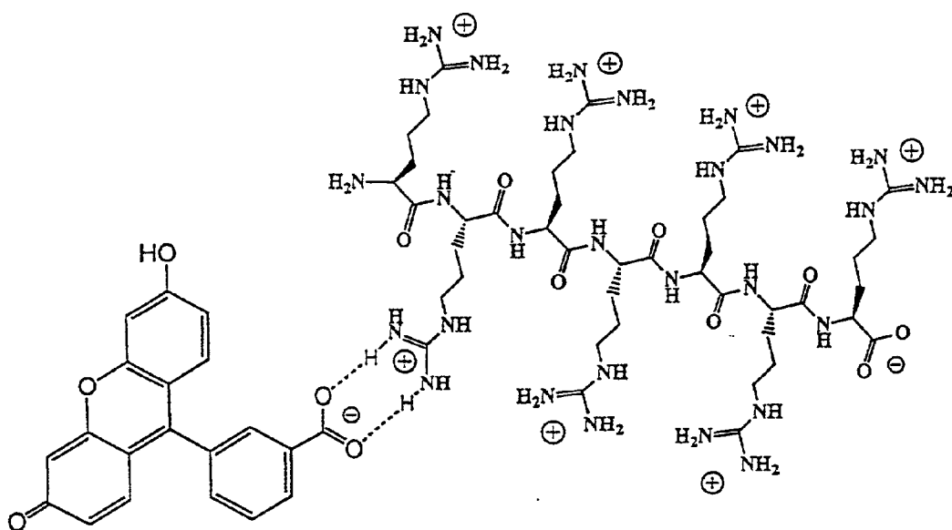
Figure 2. Diagram of the salt formed between fluorescein and a single guanidinium headgroup of a heptamer of L-arginine.
