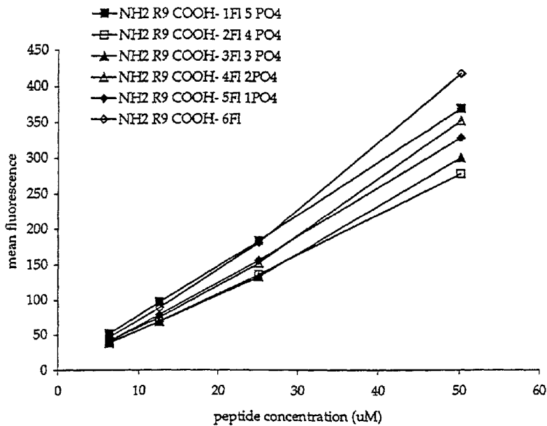
Figure 3. Staining of lymphocytes using different salts between fluorescein and nonamers of arginine. Human lymphocytes (Jurkat) were incubated with varying concentrations of each of the fluorescein-polyarginine salts for five minutes in PBS/2% fetal calf serum at room temperature. The cells were washed with PBS, exposed to 0.1% propidium iodide and analyzed by flow cytometry. The mean fluorescence of 10^4 cells is shown.
