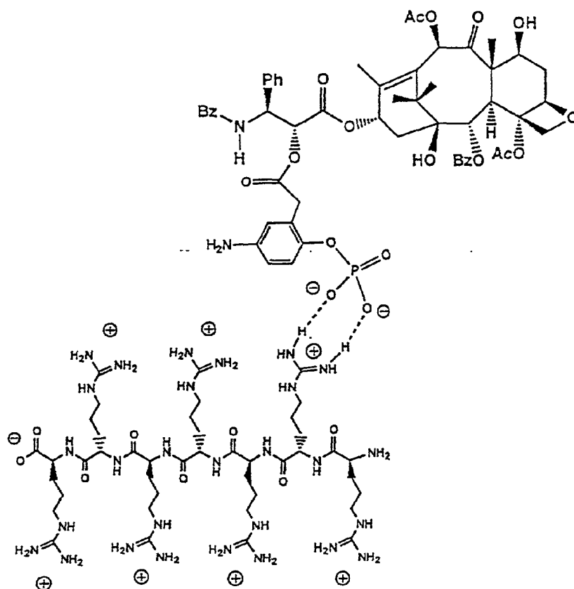
Figure 1. Diagram of the salt formed between a phosphorylated analog of taxol with a single guanidino headgroup of a heptamer of L-arginine.
