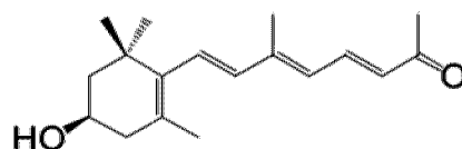
3-OH- \beta -apo-13-Carotenone (C 18 H 26 O 2 ) Zaxinone
