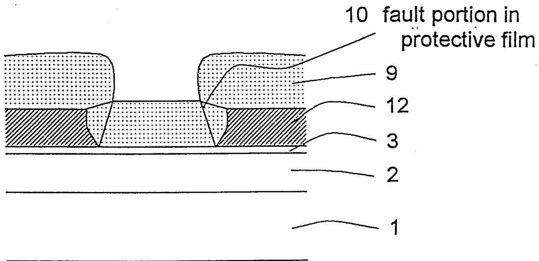
FIG. 10 (a) enlarged sectional view of heat generating portion
