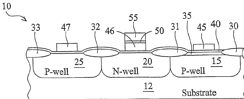
Figure. 1F (Prior Art)
