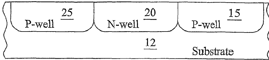
Figure. 1A (Prior Art)
