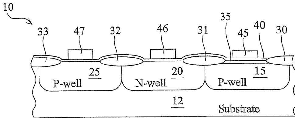
Figure. 1D (Prior Art)
