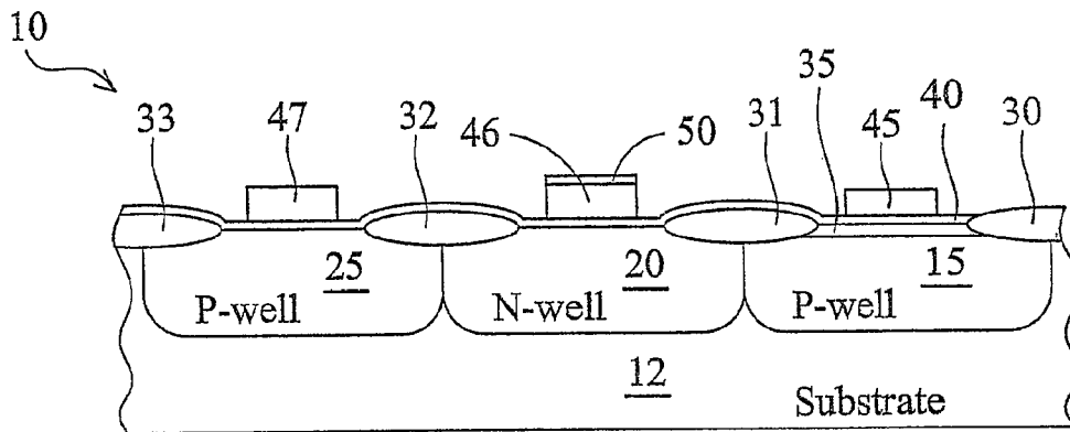
Figure. 1E (Prior Art)
