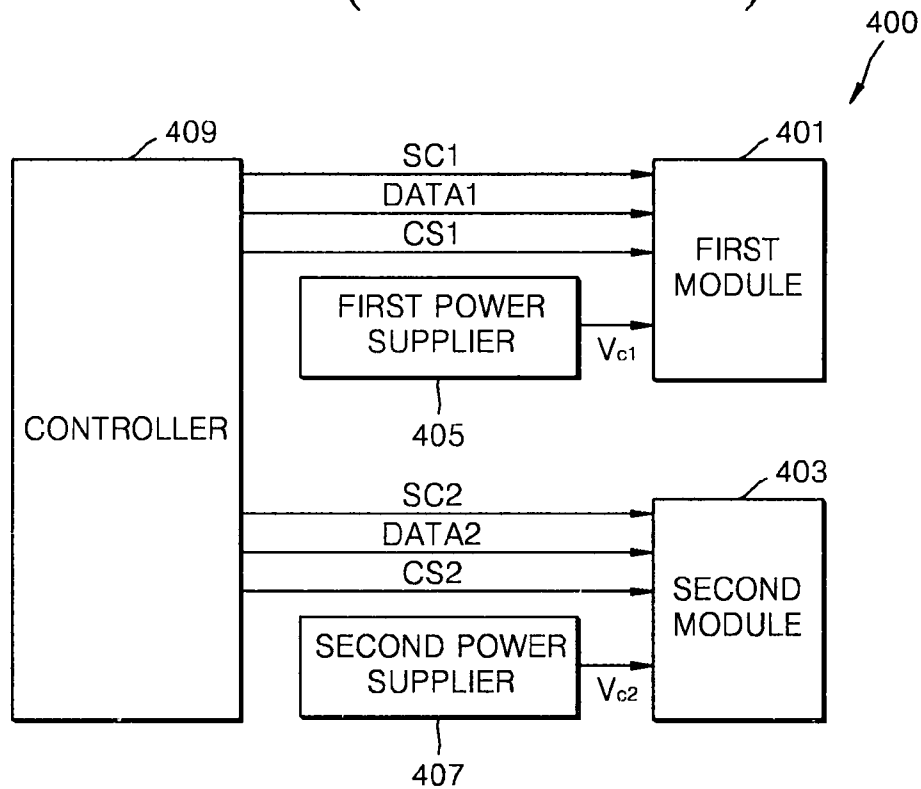
FIG. 4 (PRIOR ART)
