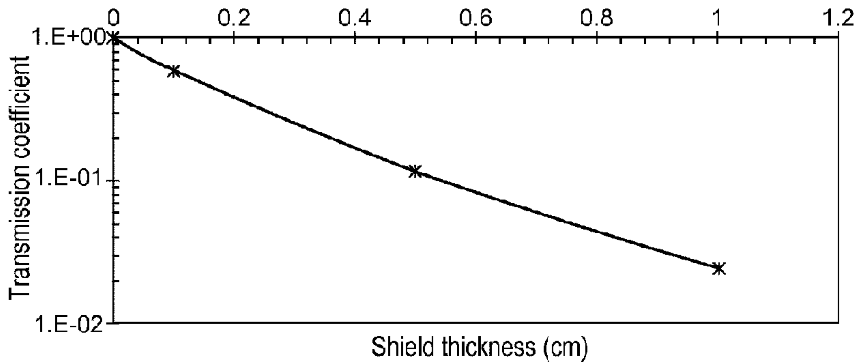
Ir-192 transmission through Iridium shielding
