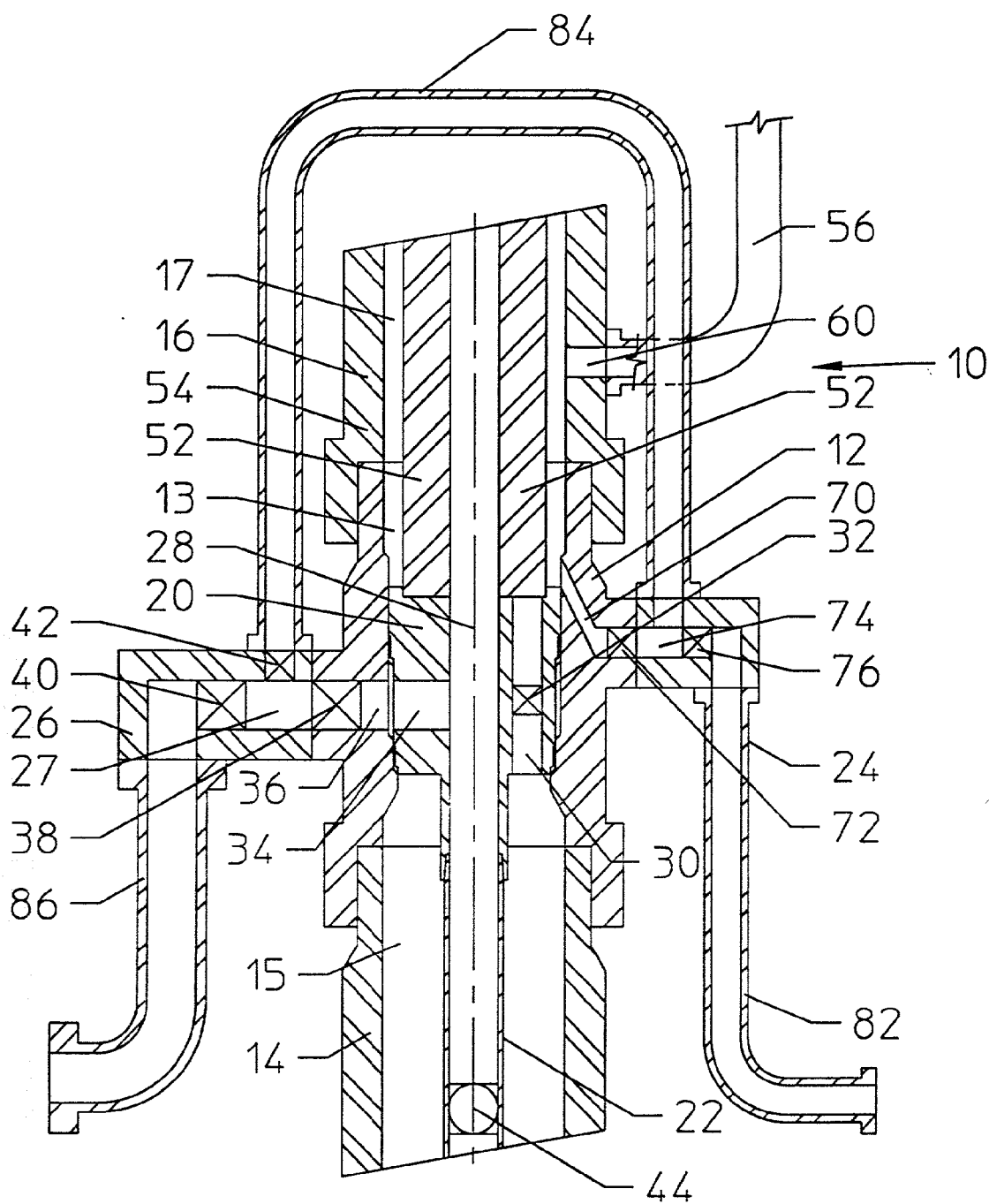
FIGURE B1 FLOW TEST
