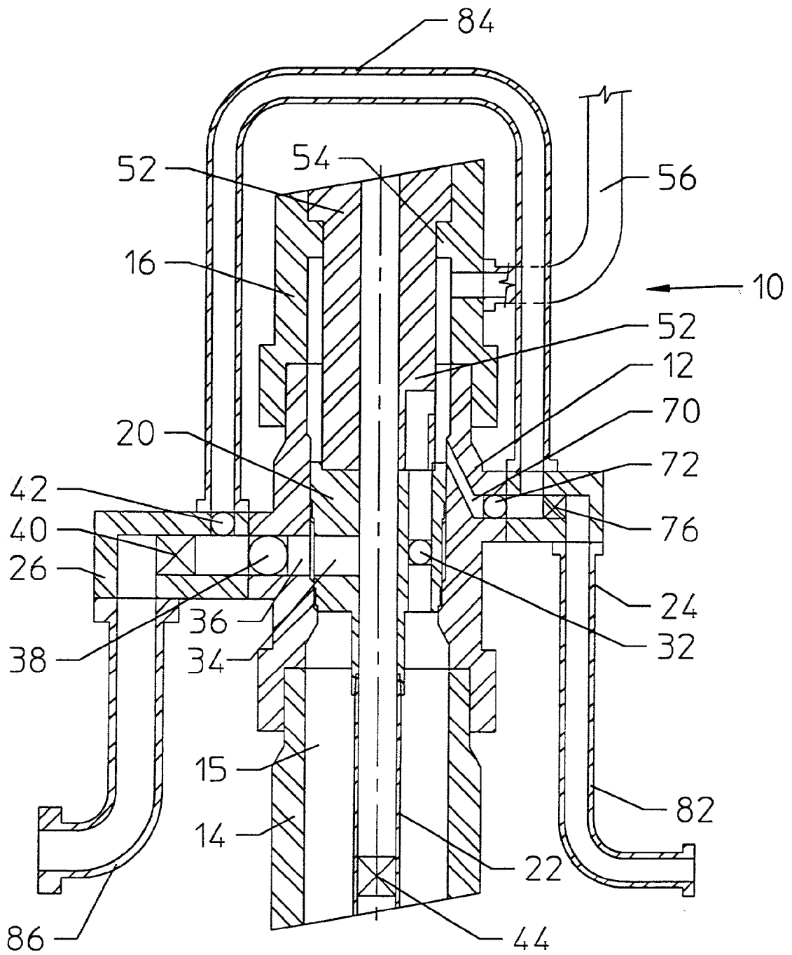
FIGURE B2 FLUSH RUNNING STRING
