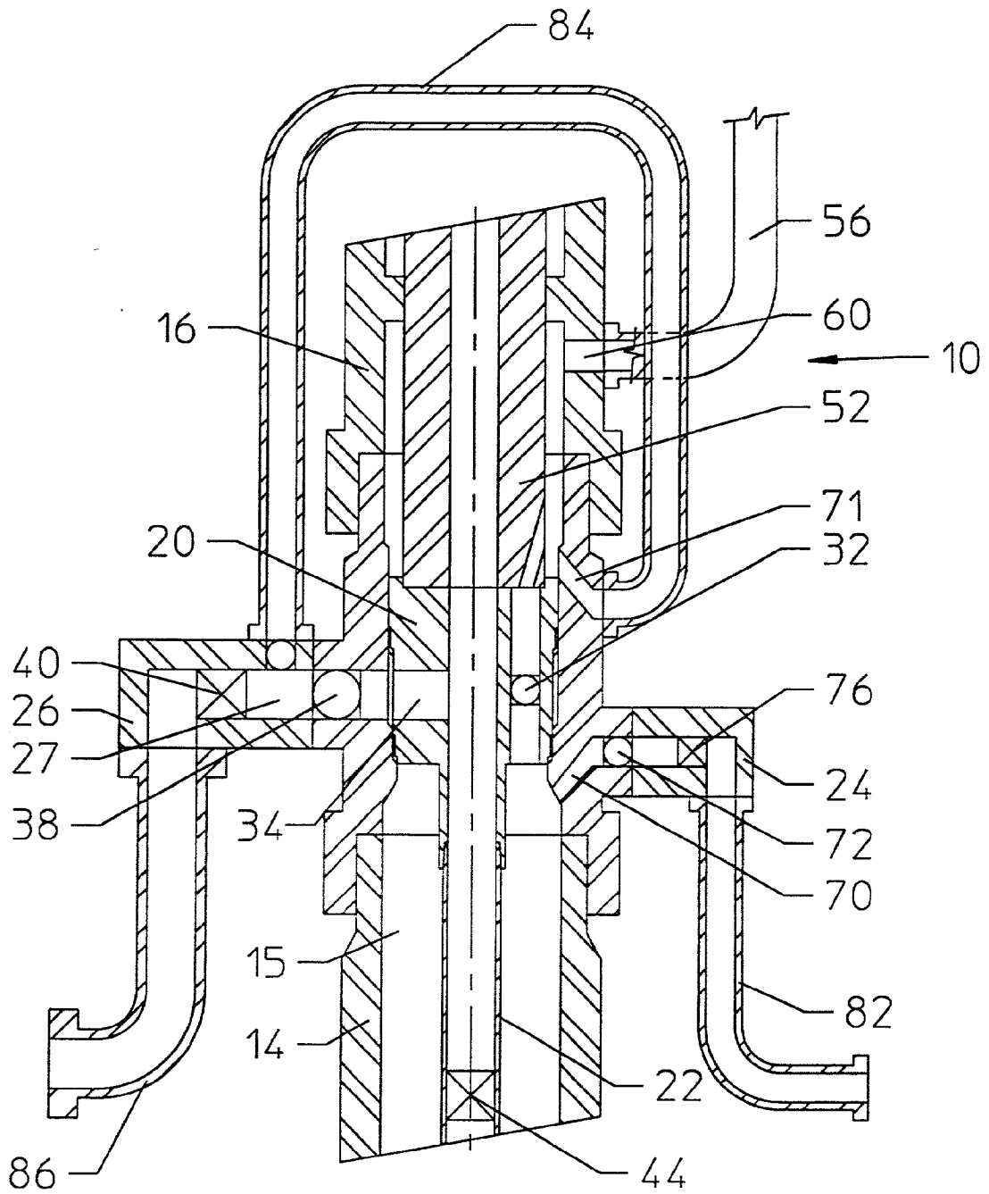
FIGURE C2 FLUSH RUNNING STRING
