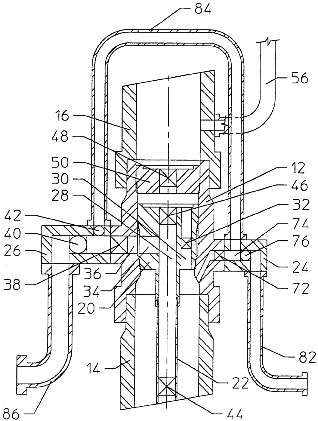
FIGURE A3 FLUSH FLOWLINES
