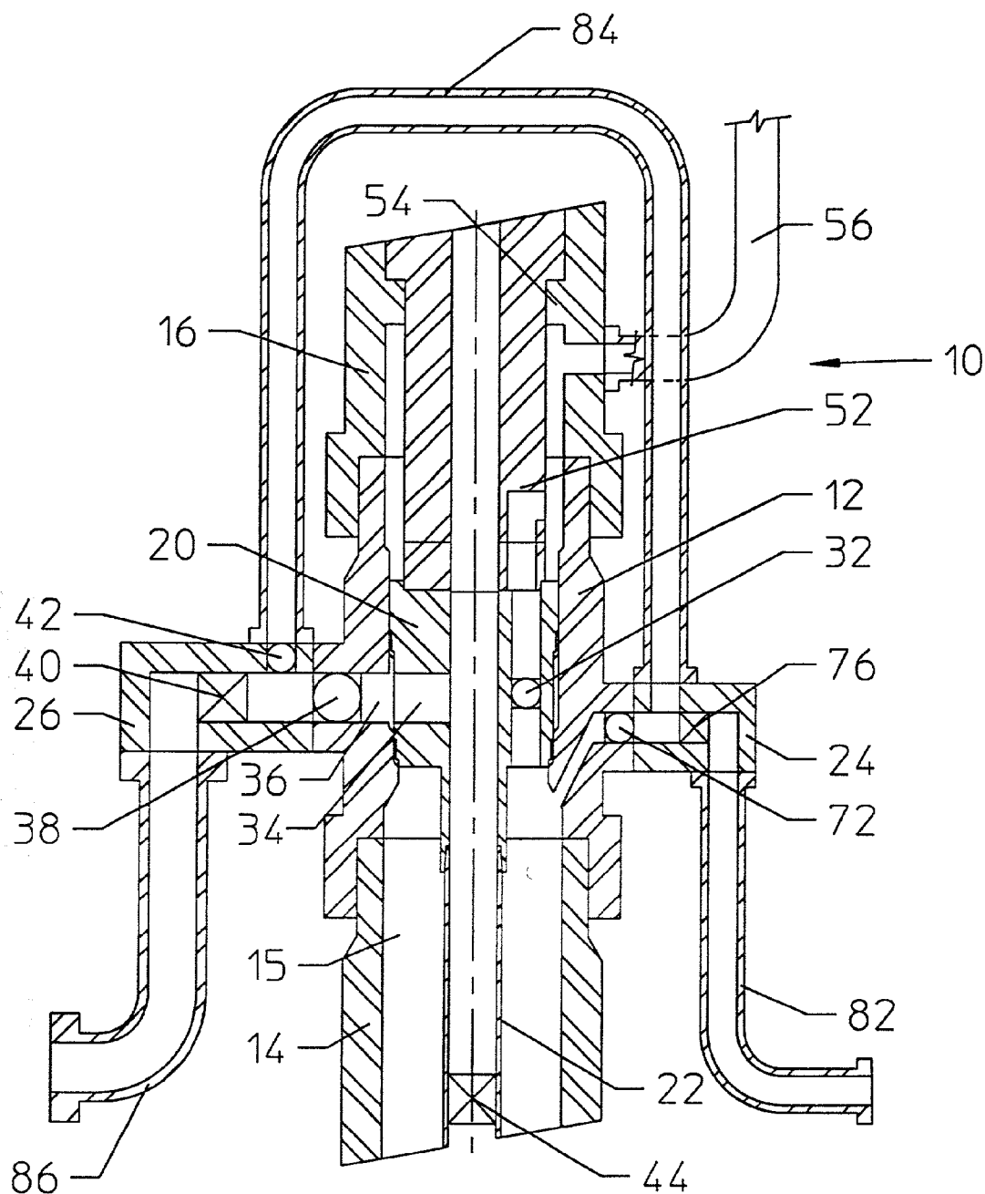
FIGURE A2 FLUSH RUNNING STRING
