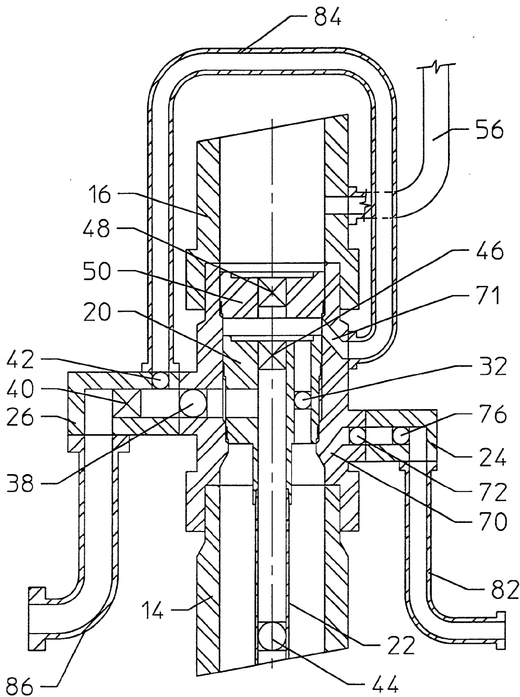
FIGURE C6 PRODUCTION CROSSOVER FLOW
