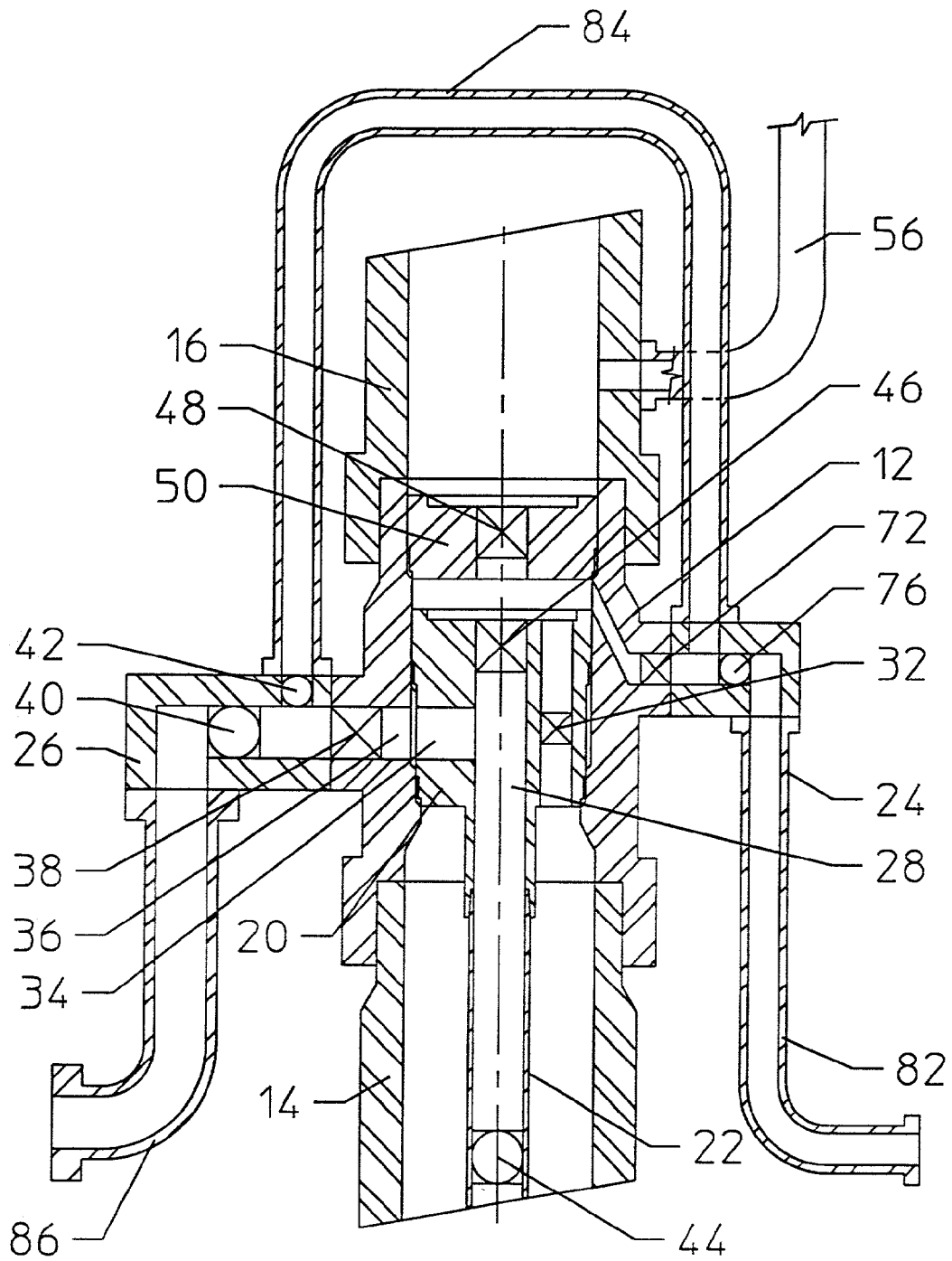
FIGURE B3 FLUSH FLOWLINES
