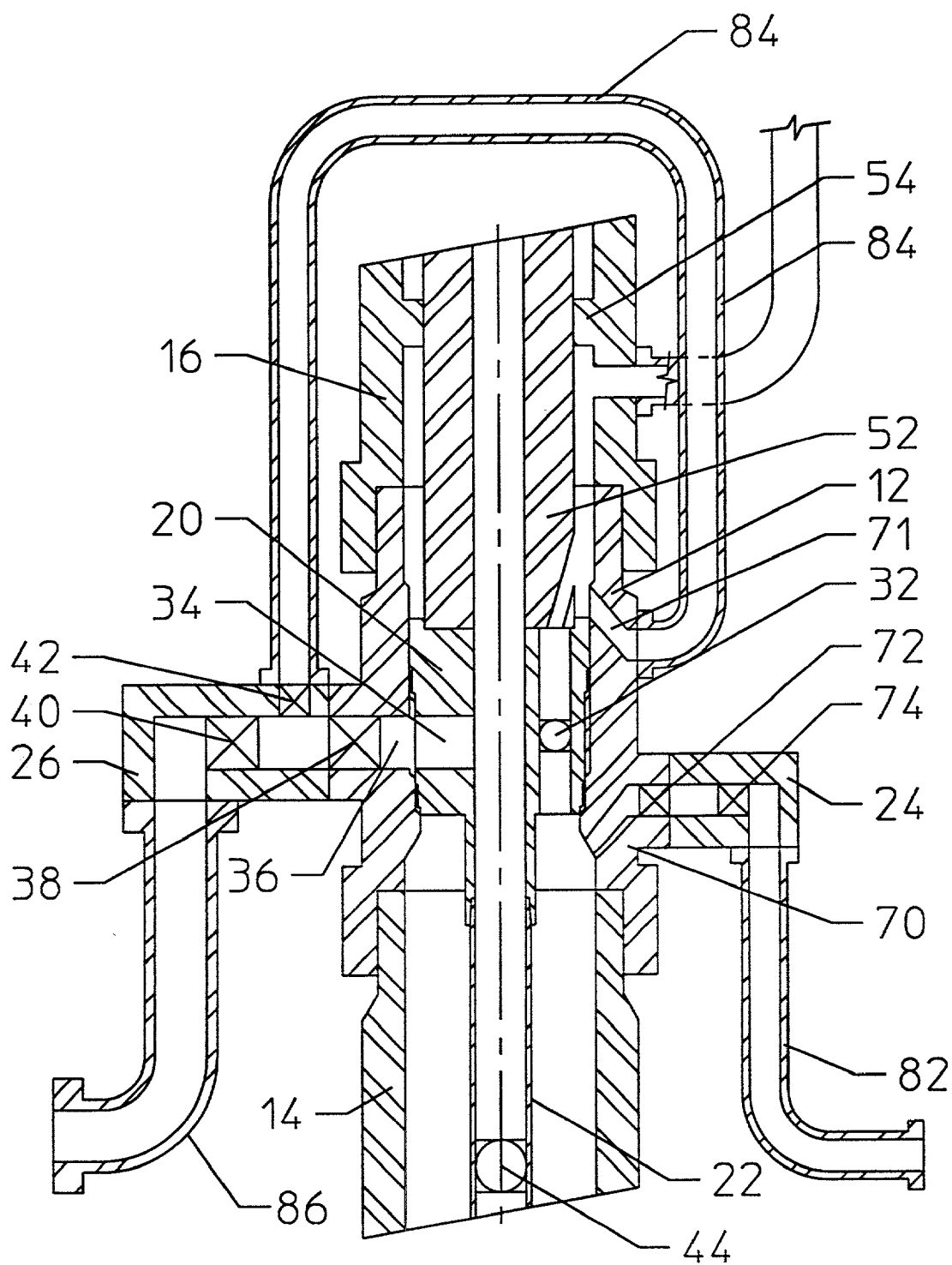
FIGURE C7 WORKOVER
