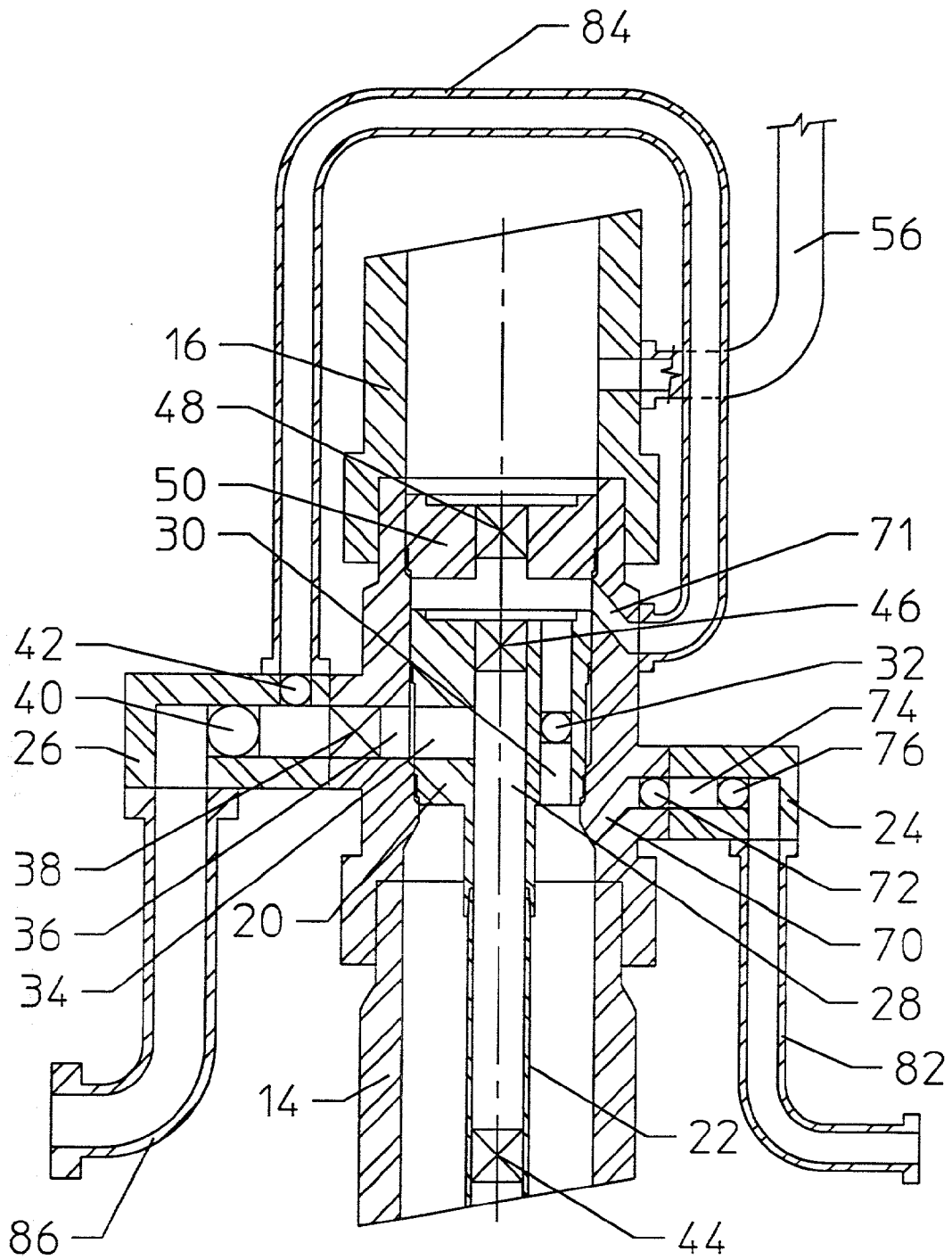
FIGURE C3 FLUSH FLOWLINES
