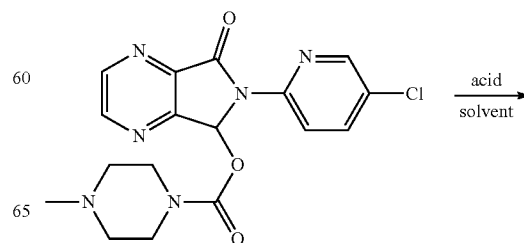
Scheme 1. Synthesis of Salt
