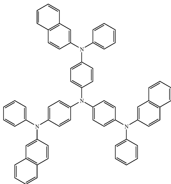
2-TNATA
