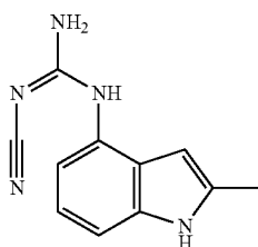
2-cyano-1-(2-methyl-1H-indol-4-yl)guanidine
