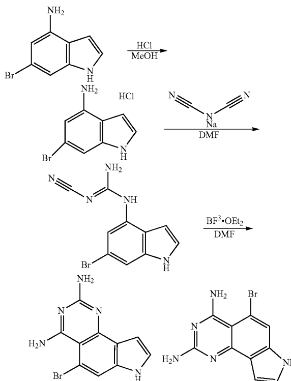
5-bromo-7H-pyrrolo[2,3-h]quinazoline-2,4-diamine
