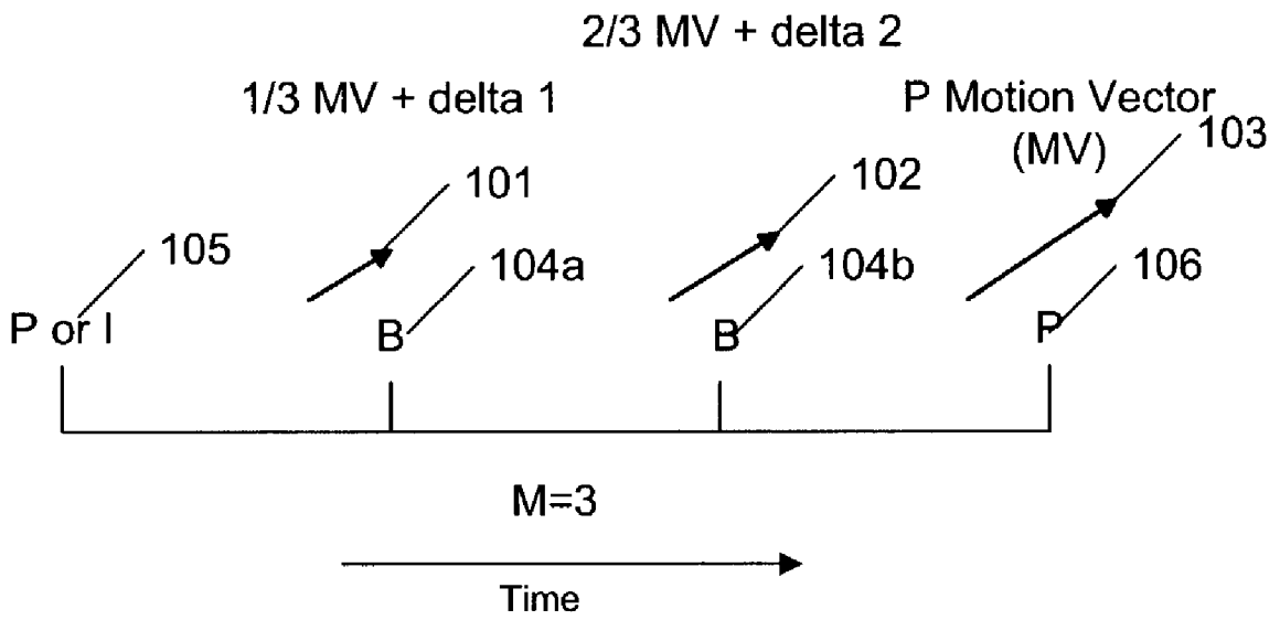
FIG. 1 Proportional Motion Vector Weighting (Prior Art)
