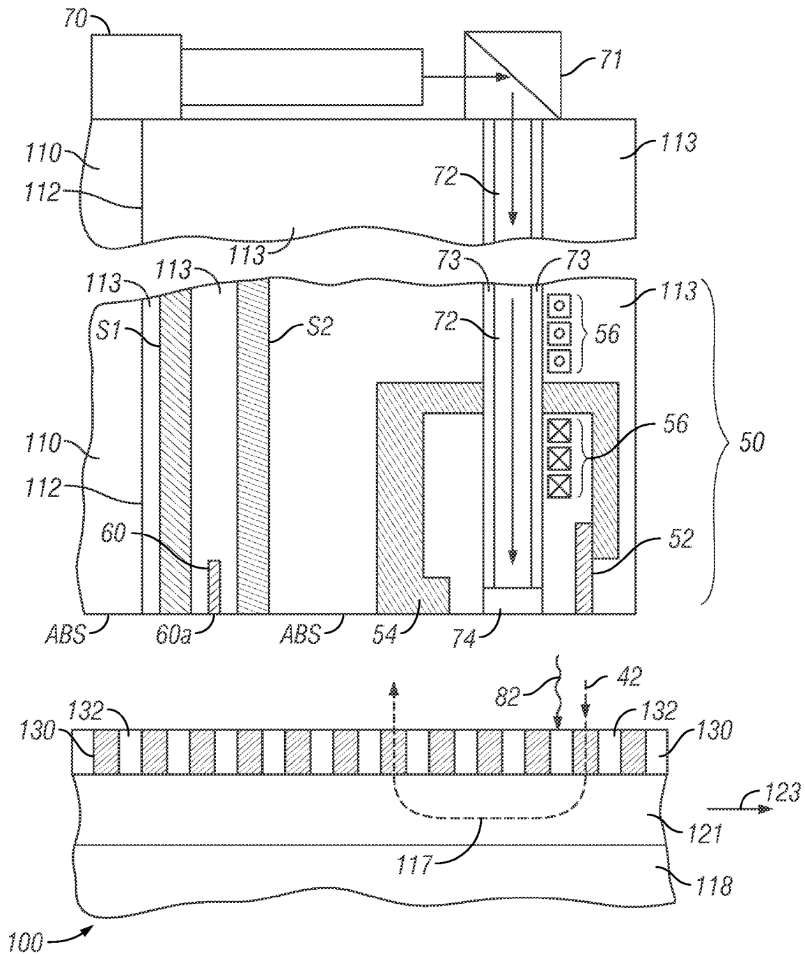
FIG. 2 (Prior Art)
