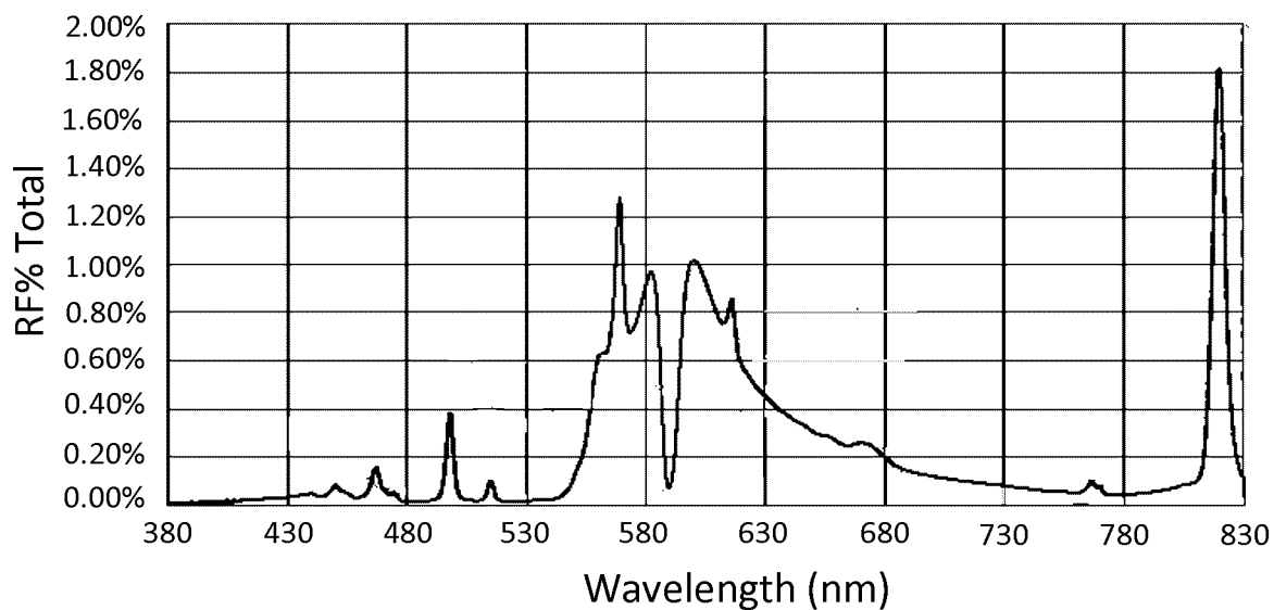
FIG. 4 (Prior art)
