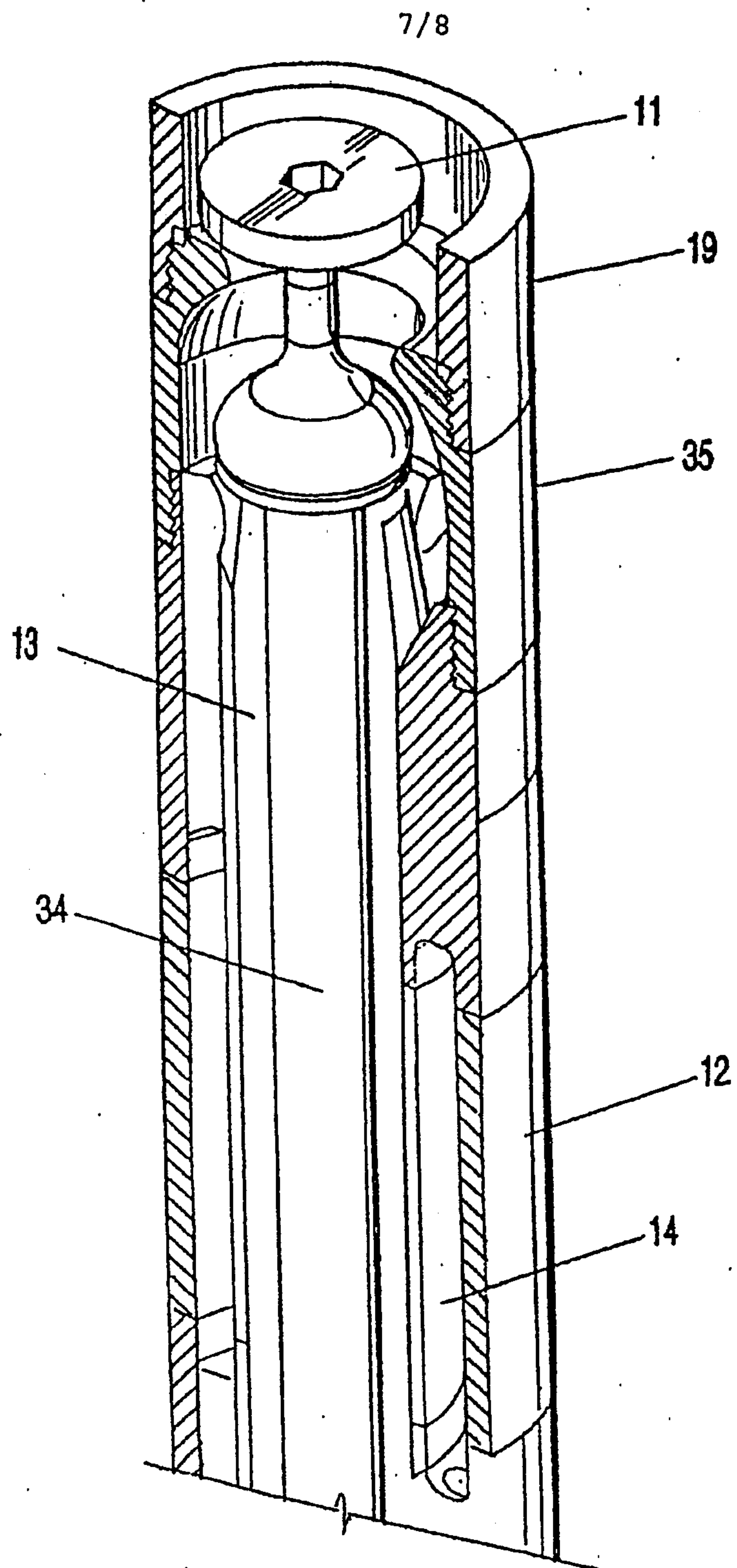
FIG-7
