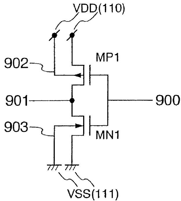
FIG.15A (PRIOR ART)
