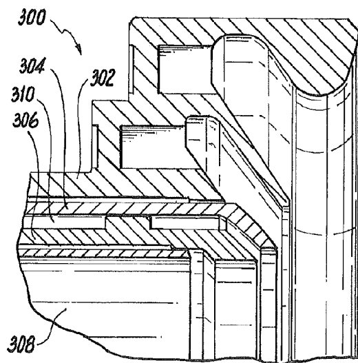
Fig. 27 (Prior Art)
