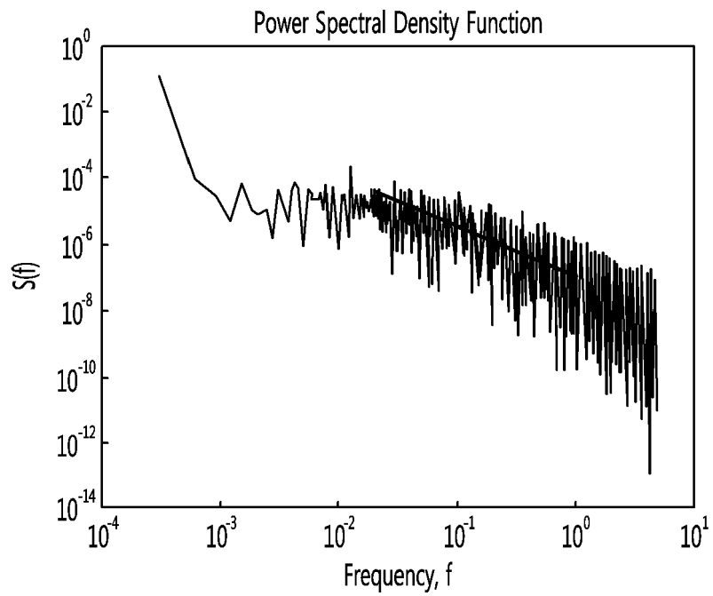
AIRFLOW FREQUENCY CHARACTERISTIC GRAPH OF NATRUAL WIND MODE (WHIRLWIND) ACCORDING TO EMBODIMENT OF INVENTION
