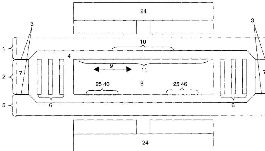
Schematic cross-section of microseismometer
