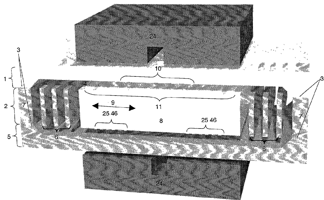
Fig. 2: 3-D View of microseismometer
