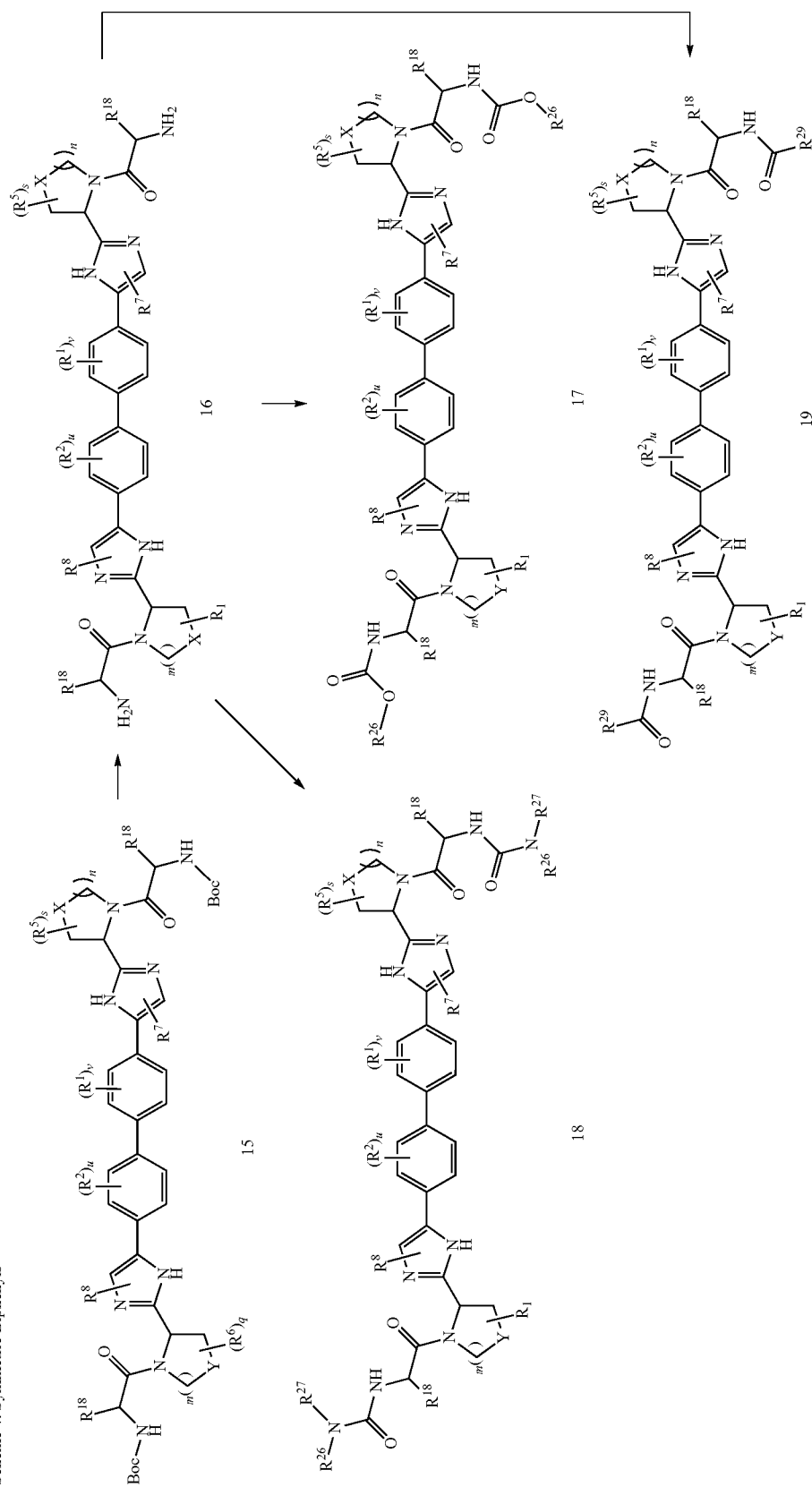
Scheme 4: Symmetric Biplenyls
