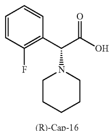
(R)-Cap-16
