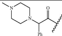
Diastereomer Cap-17c
