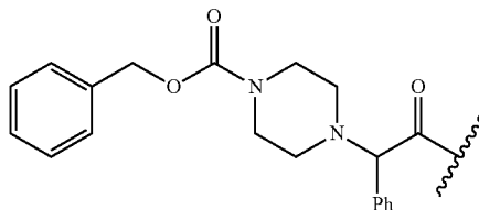
Diastereomer Cap-17a
