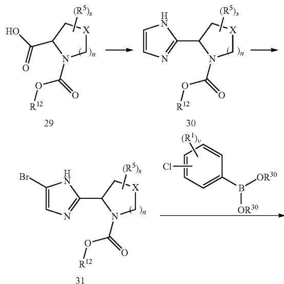
Scheme 7: Heteroaryls
