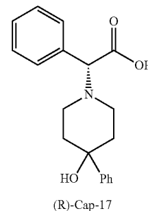
(R)-Cap-17
