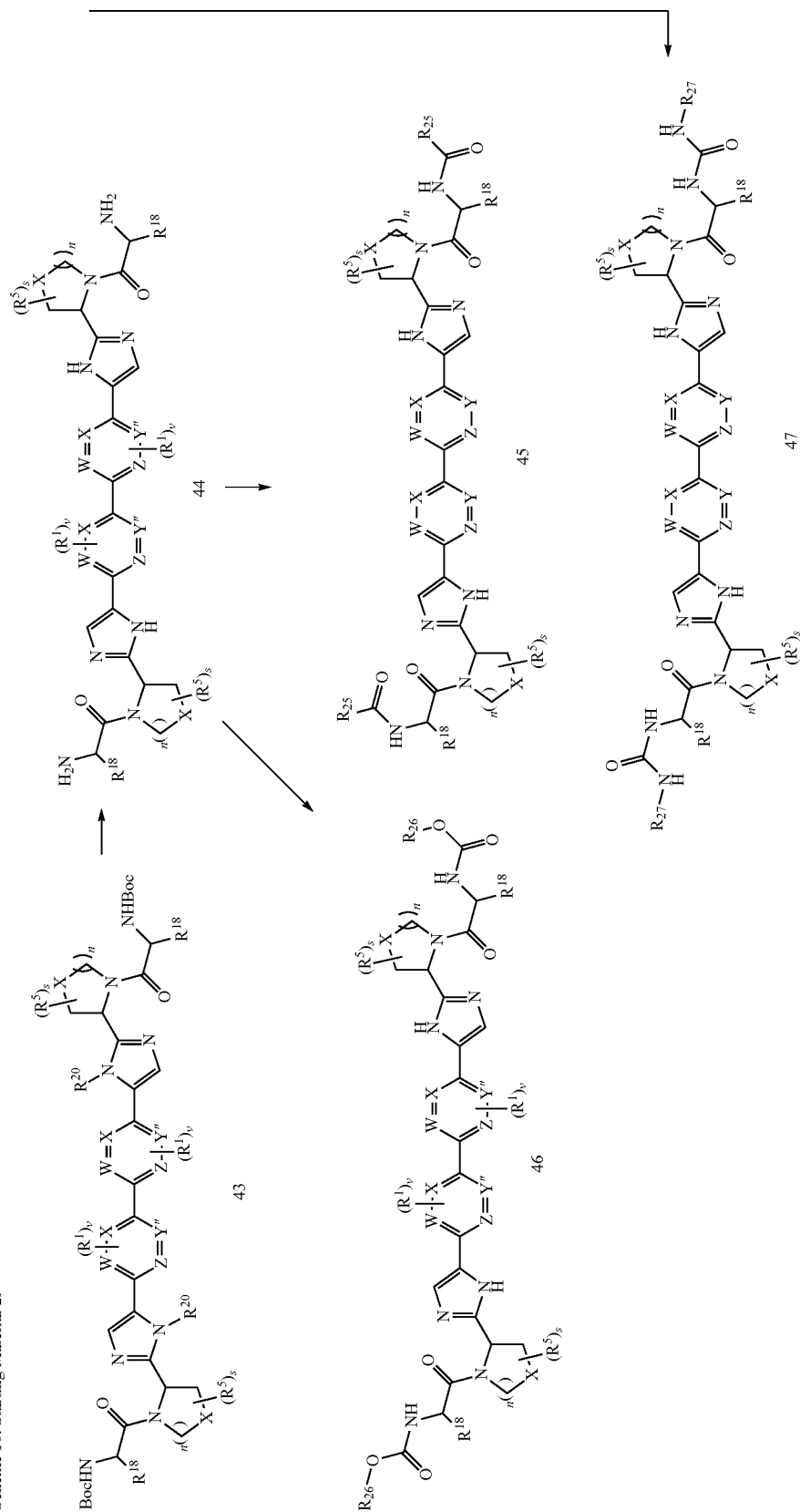
Scheme 10: Starting Material 29
