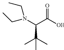
Cap-74x
