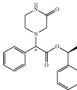
Intermediate-17b
