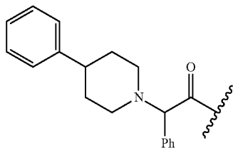
Diastereomer Cap-17d
