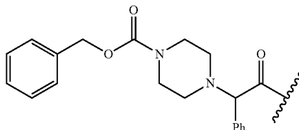
Diastereomer Cap-17a
