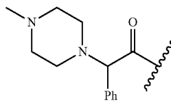
Diastereomer Cap-17c
