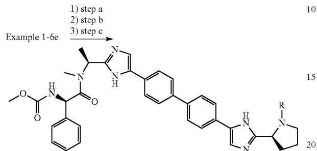
Example 131.1-1 to 131.1-2
