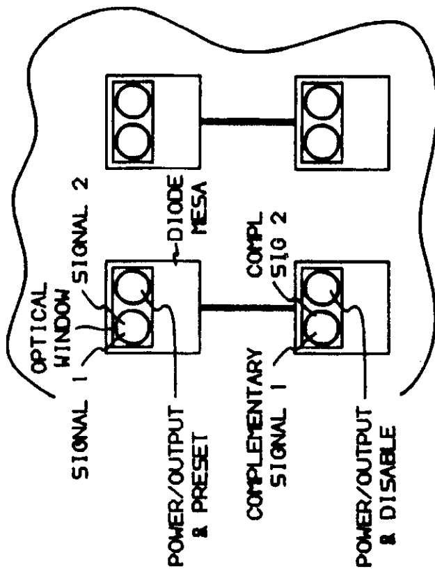
S-SEED ARRAY
