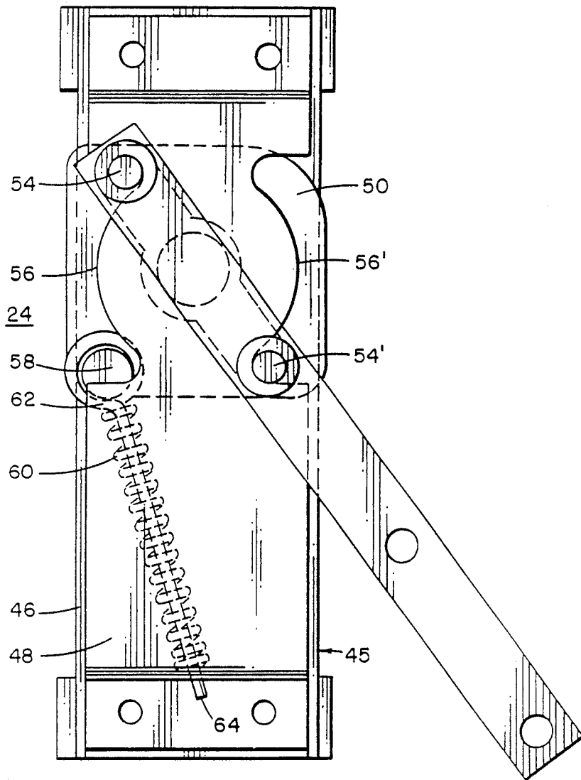
FIG. 3 (PRIOR ART)
