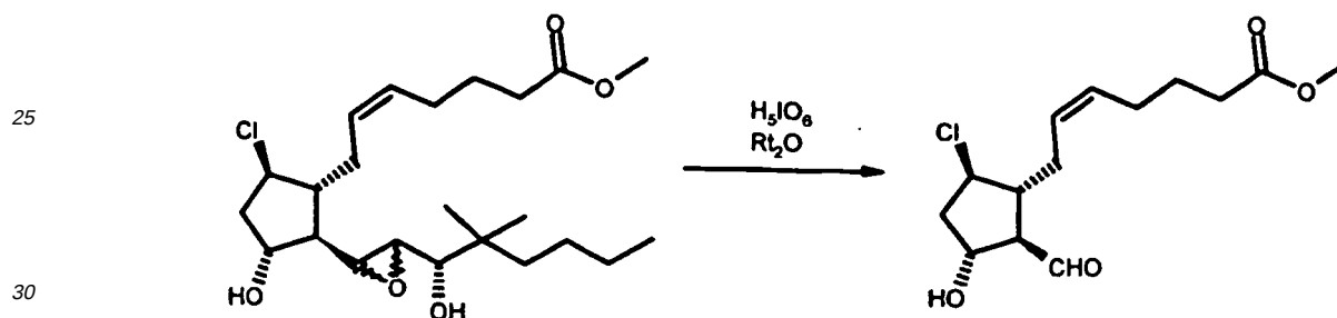
1c) Methyl (5Z)-(9R, 11 R)-9-chloro-11-[(2H)-tetrahydropyran-2-yloxy]-14,15,16,17,18,19,20-heptanor-12-oxo-5-prostenoate
