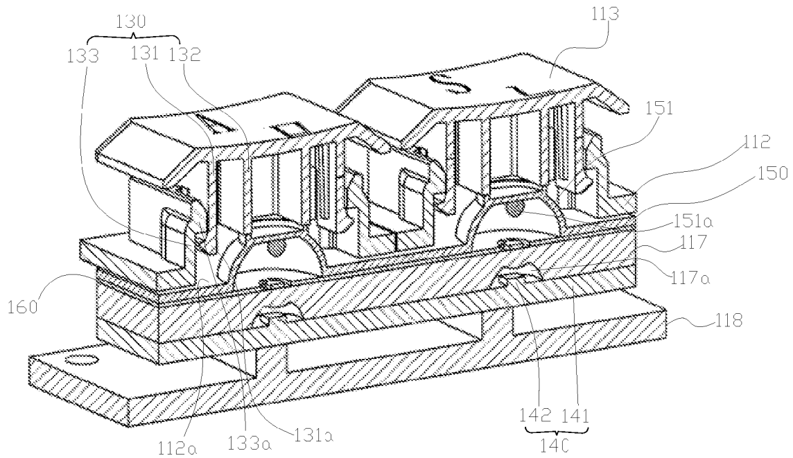
FIG. 9 (Prior Art)
