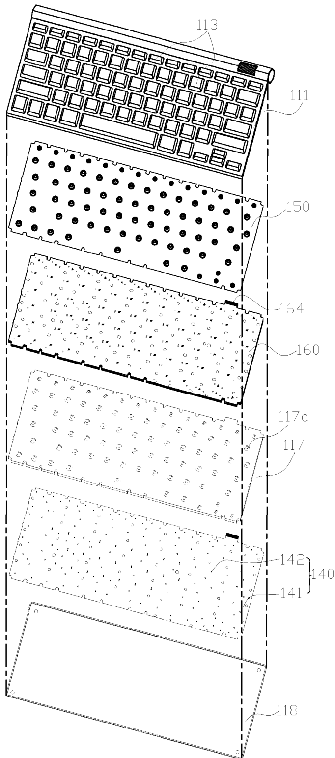
FIG. 8 (Prior Art)
