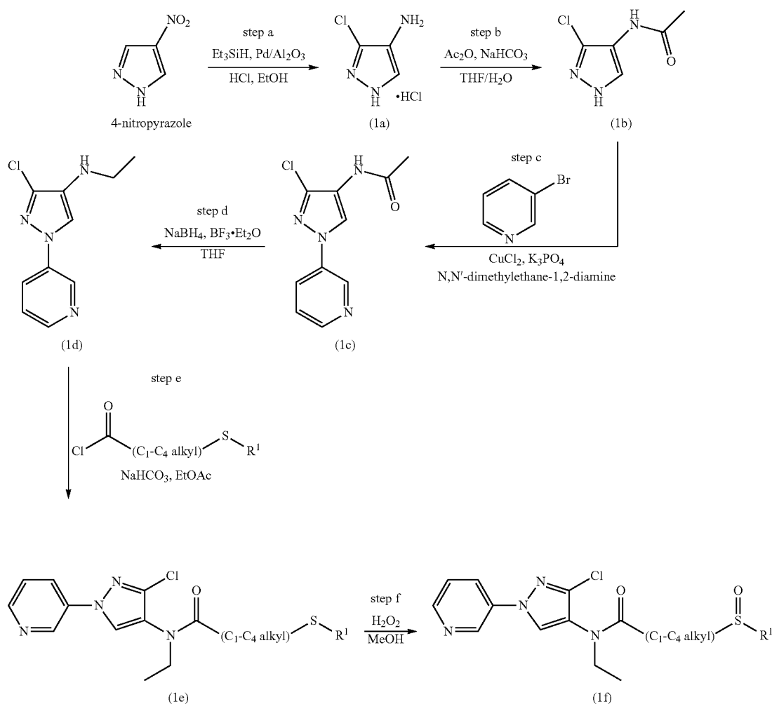
Scheme 1
