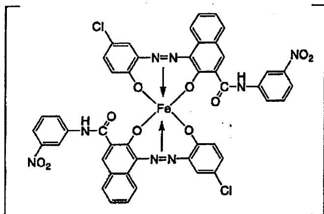
[0154] Azo-based iron complex compound (4)
