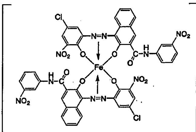
[0155] Azo-based iron complex compound (5)
