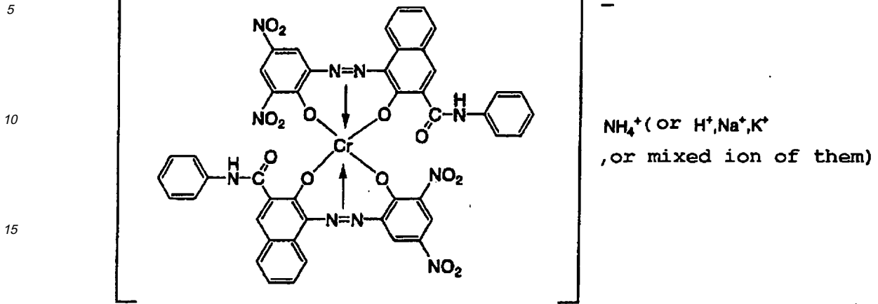
[0160] Azo-based iron complex compound (9)
