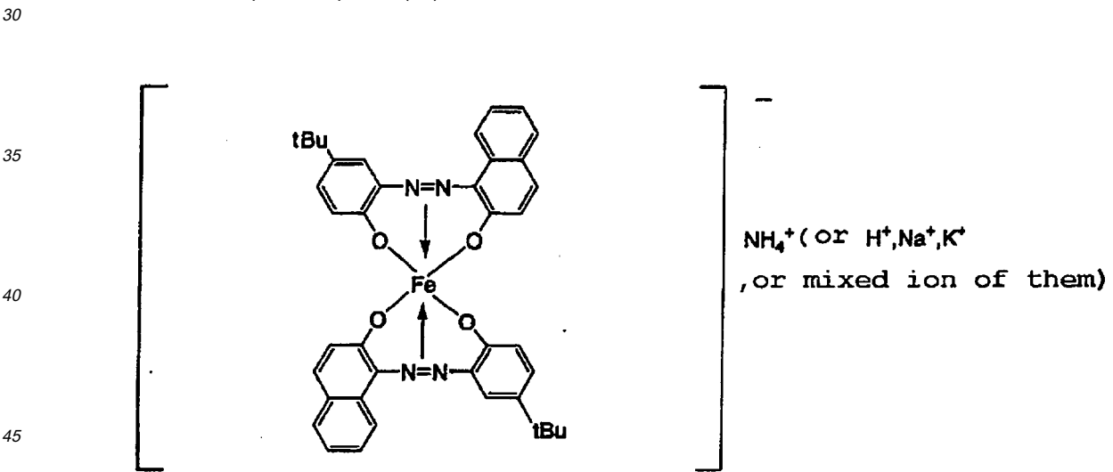
Azo-based iron complex compound (13)
