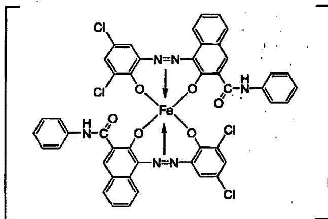
[0153] Azo-based iron complex compound (3)
