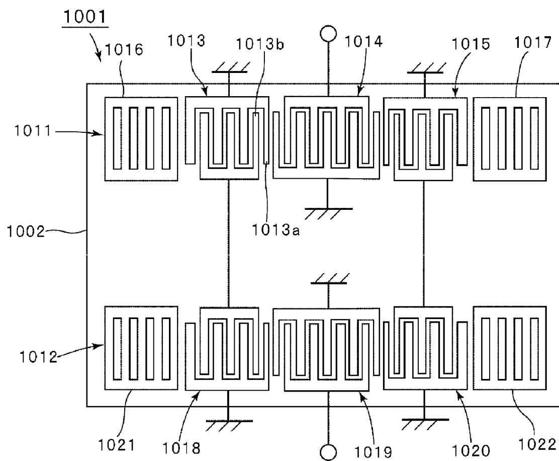
FIG. 7 PRIOR ART
