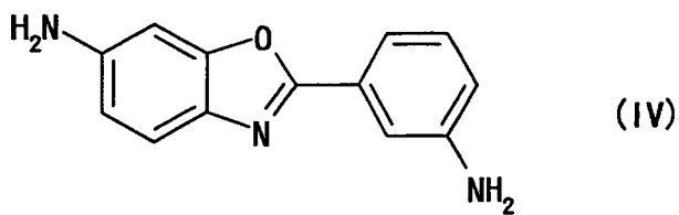
6-amino-2-(m-aminophenyl)benzoxazole
