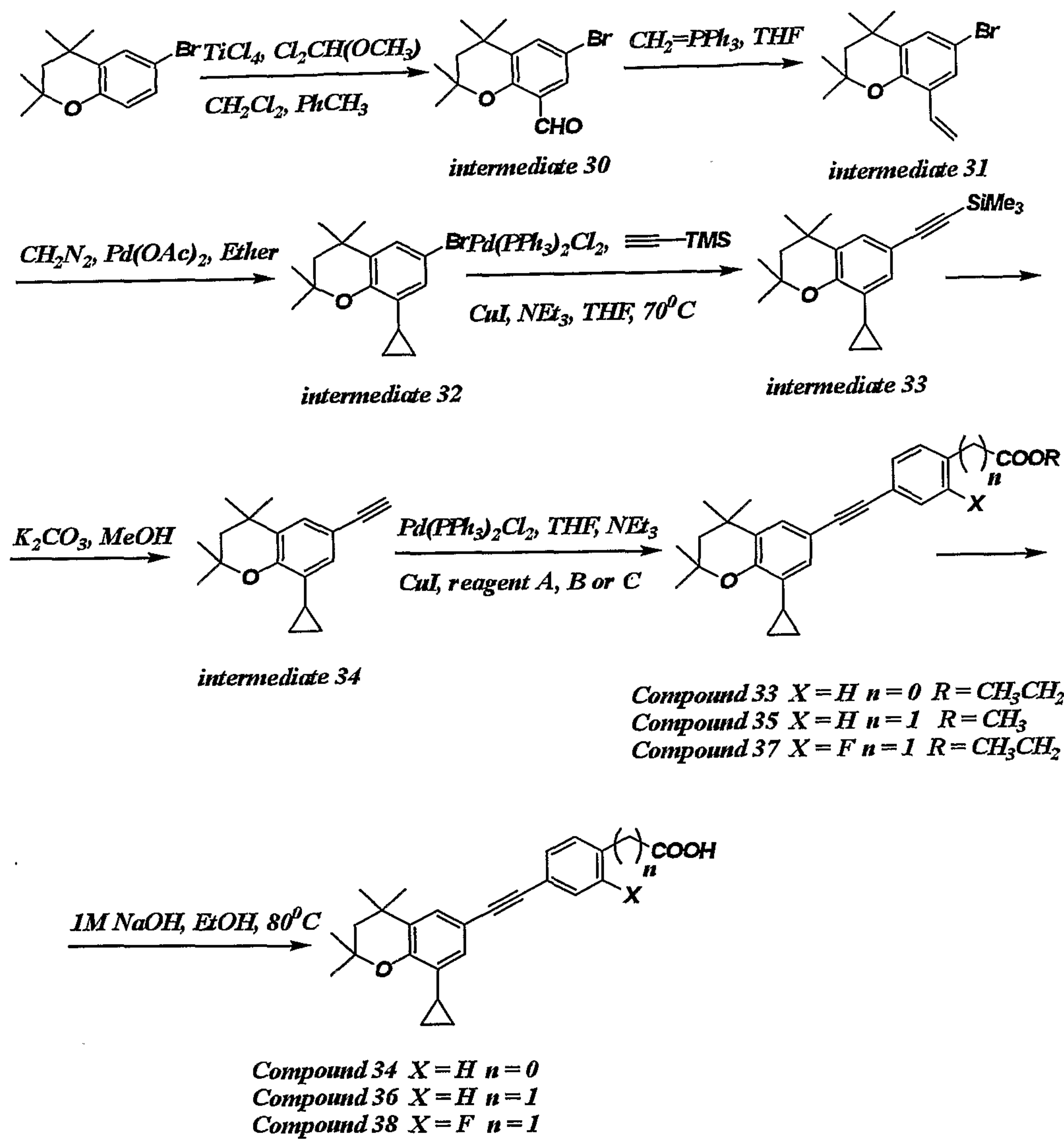
REACTION SCHEME 6
