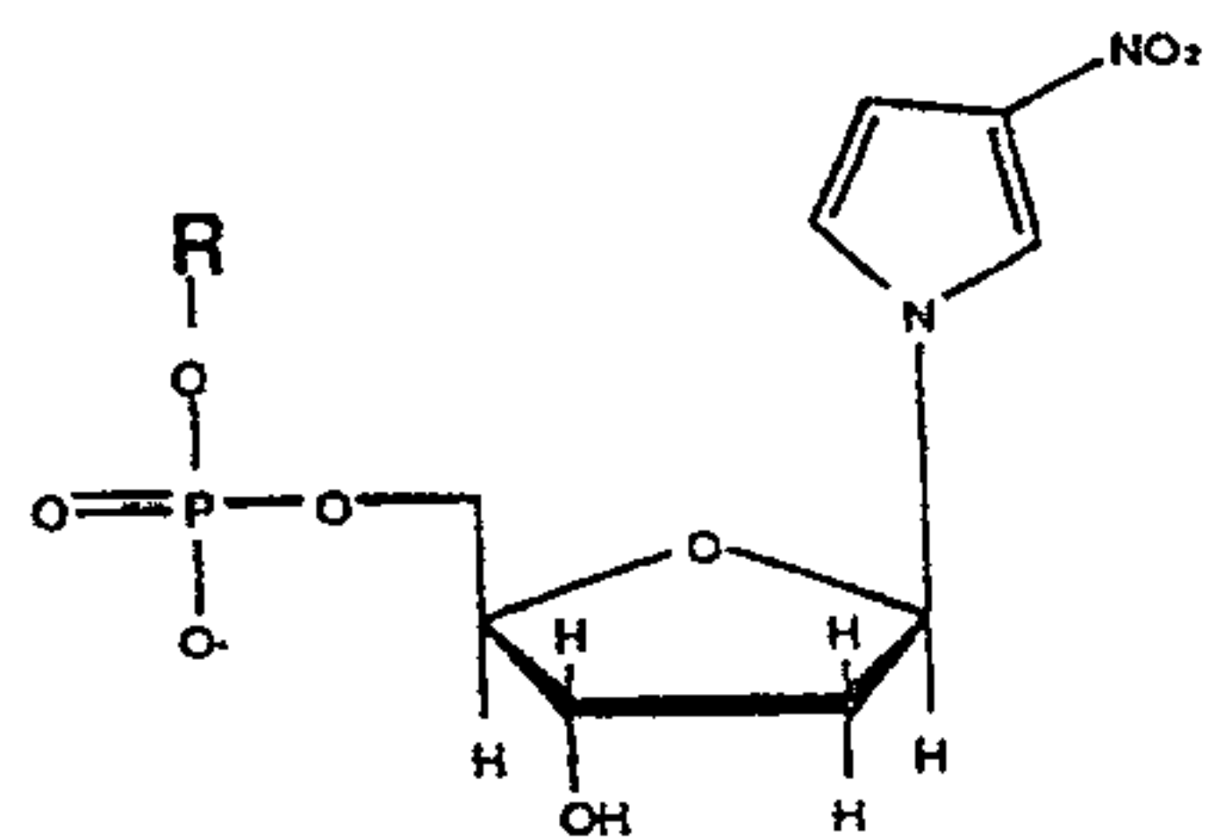
3-nitropyrrole
