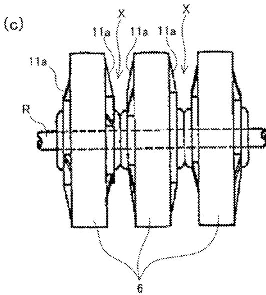
Fig. 8c PRIOR ART
