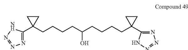
1,9-Bis-[1-(1H-tetrazol-5-yl)-cyclopropyl]-nonan-5-ol
