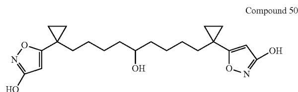
1,9-Bis-[1-(3-hydroxy-isoxazol-5-yl)-cyclopropyl]-nonan-5-ol
