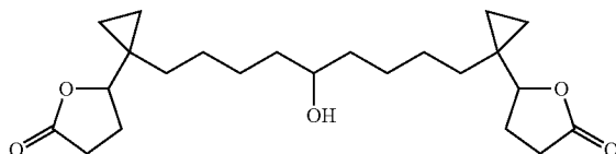
1,9-Bis-[1-(2-oxo-tetrahydrofuran-5-yl)-cyclopropyl]-nonan-5-ol
