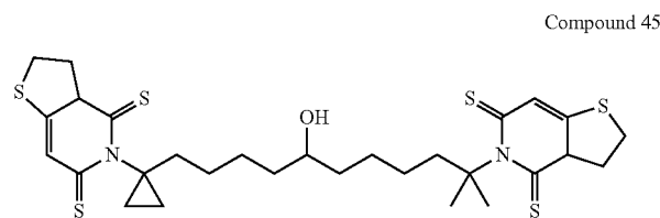
2,12-Bis-(4,6-dithio-2,3,3a,6-tetrahydro-4H-thieno[3,2-c]pyridin-5-yl)-2-methyl-12-(cyclopropyl)-7-hydroxy-dodecane
