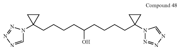
1,9-Bis-(1-tetrazol-1-yl-cyclopropyl)-nonan-5-ol
