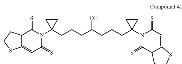
1,7-Bis-(4,6-dithio-2,3,3a,6-tetrahydro-4H-thieno[3,2-c]pyridin-5-yl)-1,7-bis-(cyclopropyl)-6-hydroxy-heptane
