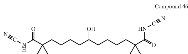
1,7-Bis-(1-dicyanimido-cyclopropyl)-5-hydroxy-nonane
