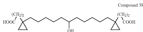
3-(1-(11-(1-(2-Carboxy-ethyl)-cyclopropyl)-6-hydroxy-undecyl)-cyclopropyl)-propionic acid
