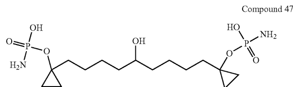
1,7-Bis-(1-phosponamido-cyclopropyl)-5-hydroxy-nonane
