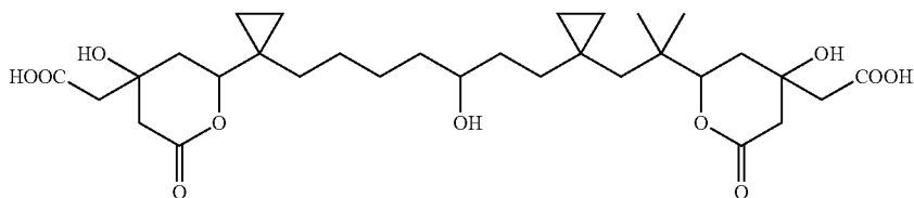
1,9-Bis {1-[9-(4-carboxymethyl-4-hydroxy-6-oxo-tetrahydro-pyran-2-yl)-(cyclopropyl)]-5-hydroxy-nonane
