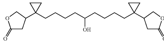
1,9-Bis-[1-(2-oxo-tetrahydrofuran-4-yl)-cyclopropyl]-nonan-5-ol
