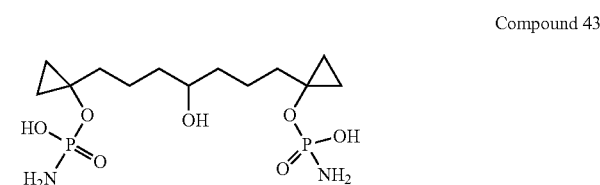
1,7-Bis-(1-phosponamid-cyclopropyl)-4-hydroxy-heptane
