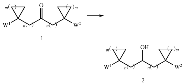
Scheme 1: Synthesis of compounds of formula 2 and 4
