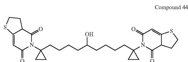
2,9-Bis-(4,6-dioxo-2,3,3a,6-tetrahydro-4H-thieno[3,2-c]pyridin-5-yl)-2,9-bis-(cyclopropyl)-5-hydroxy-nonane
