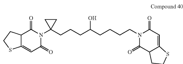
1,7-Bis-(4,6-dioxo-2,3,3a,6-tetrahydro-4H-thieno[3,2-c]pyridin-5-yl)-1-(cyclopropyl)-6-hydroxy-heptane
