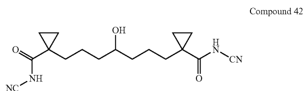
1,7-Bis-(1-dicyanimido-cyclopropyl)-4-hydroxy-heptane
