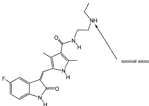
Des-ethyl Sunitinib
