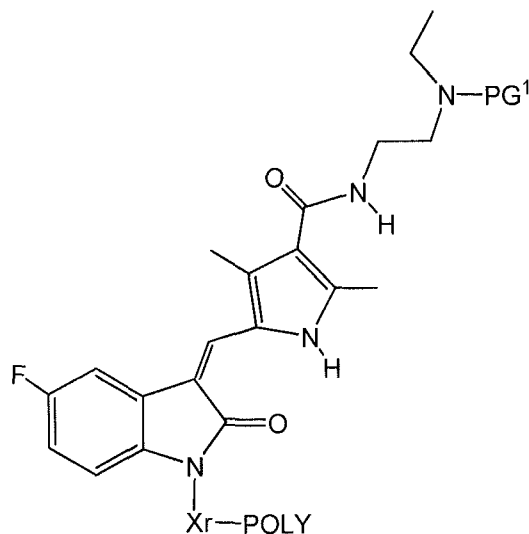
(Formula I-C-PG 1 )
