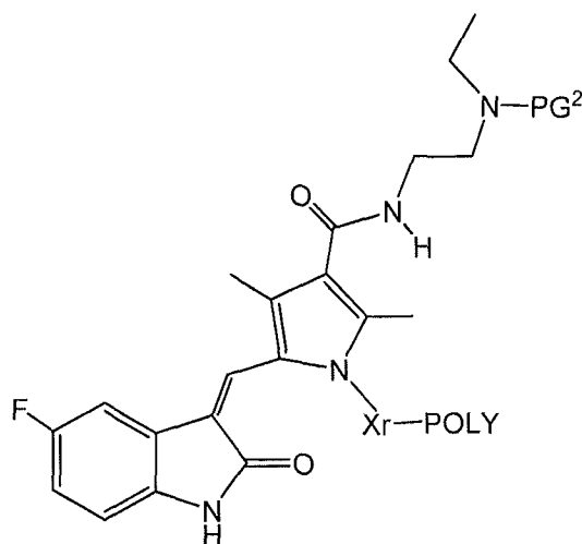
(Formula I-C-PG 2 )
