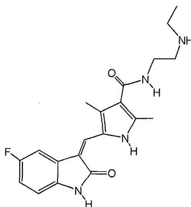
Des-ethyl Sunitinib
