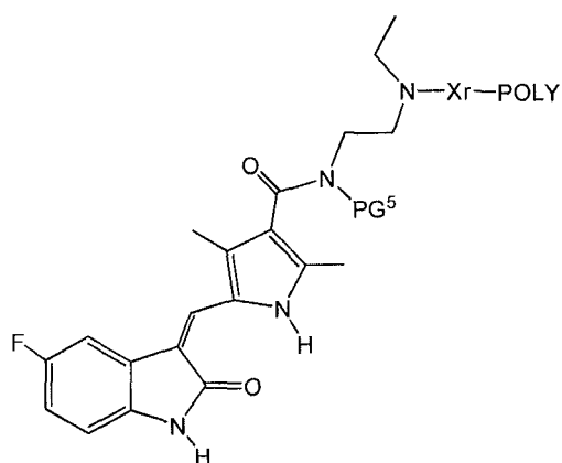
(Formula I-C-PG 5 )
