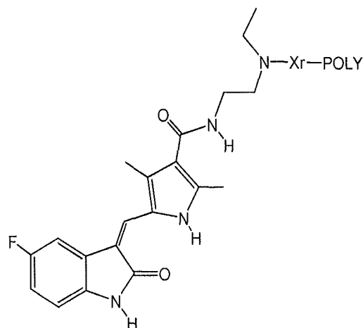
(Formula I-C)
