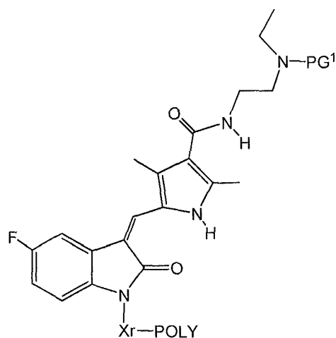
(Formula I-C-PG 1 )
