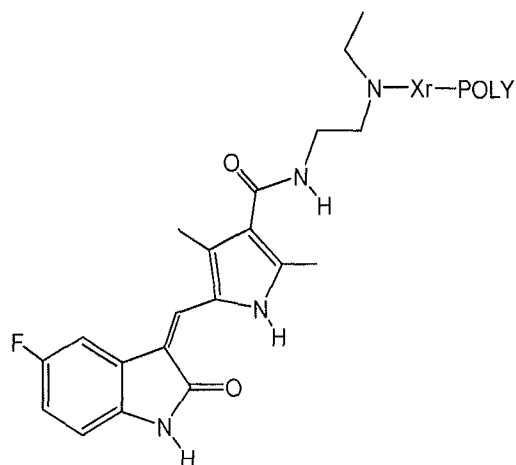
(Formula I-C)
