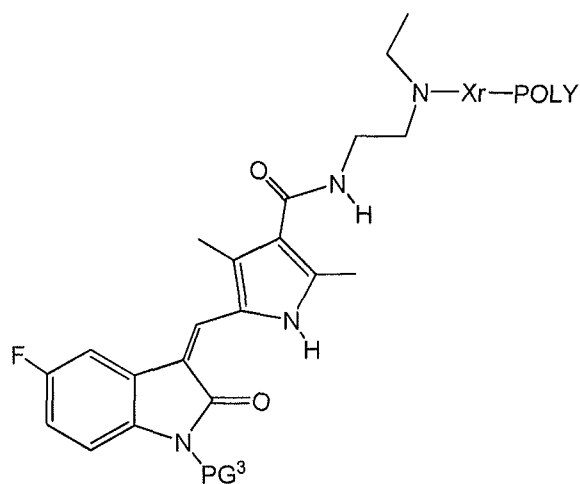
(Formula I-C-PG 3 )
