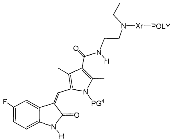
(Formula I-C-PG 4 )
