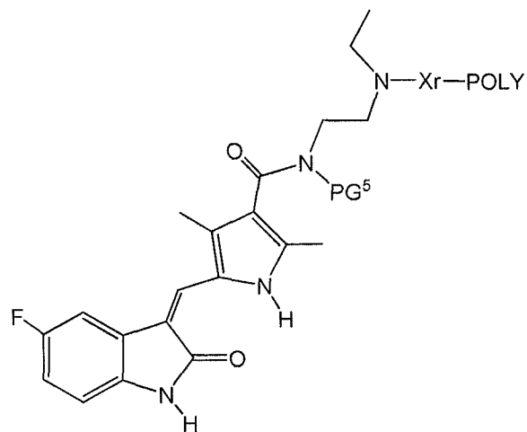
(Formula I-C-PG 5 )
