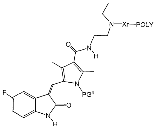
(Formula I-C-PG 4 )
