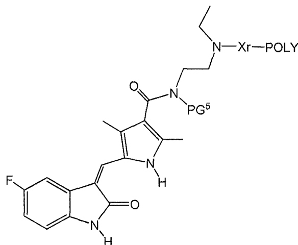
(Formula I-C-PG 5 )
