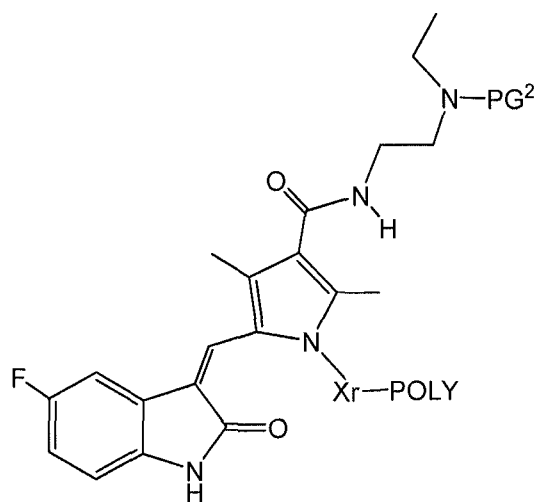
(Formula I-C-PG 2 )
