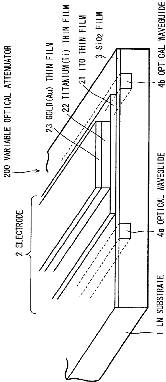
FIG. 2 PRIOR ART
