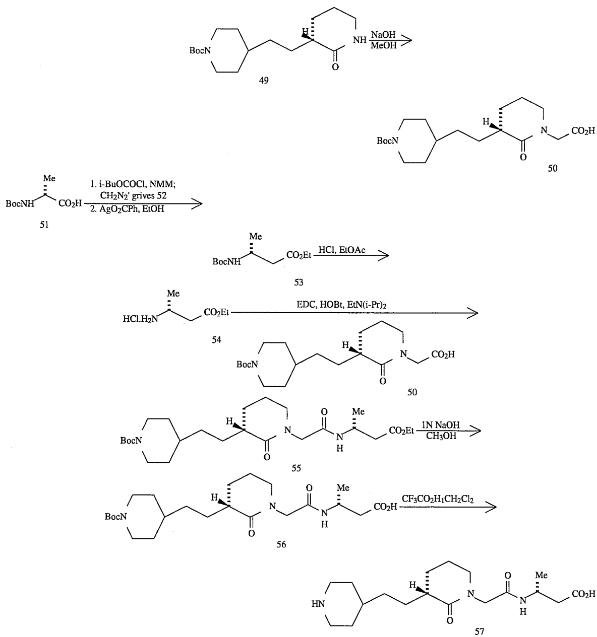
SCHEME 7
