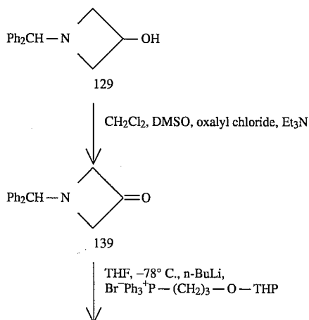
SCHEME 17
