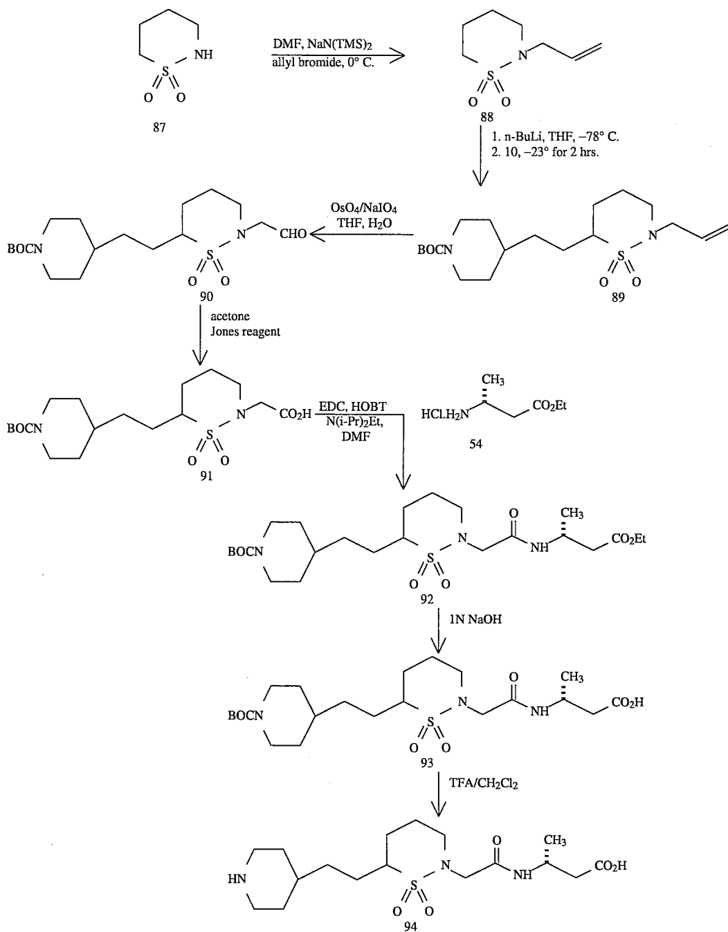
SCHEME 11
