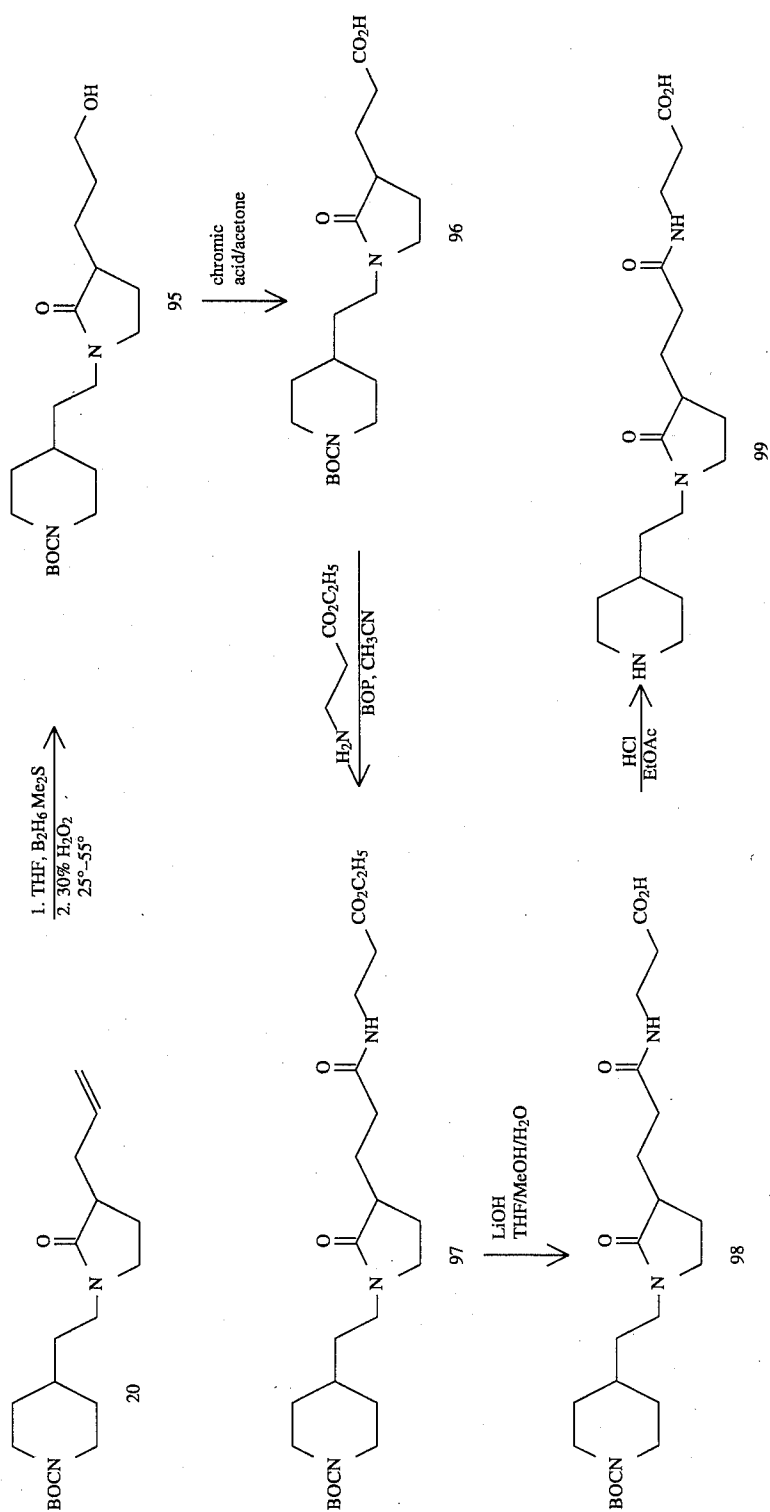
SCHEME 12
