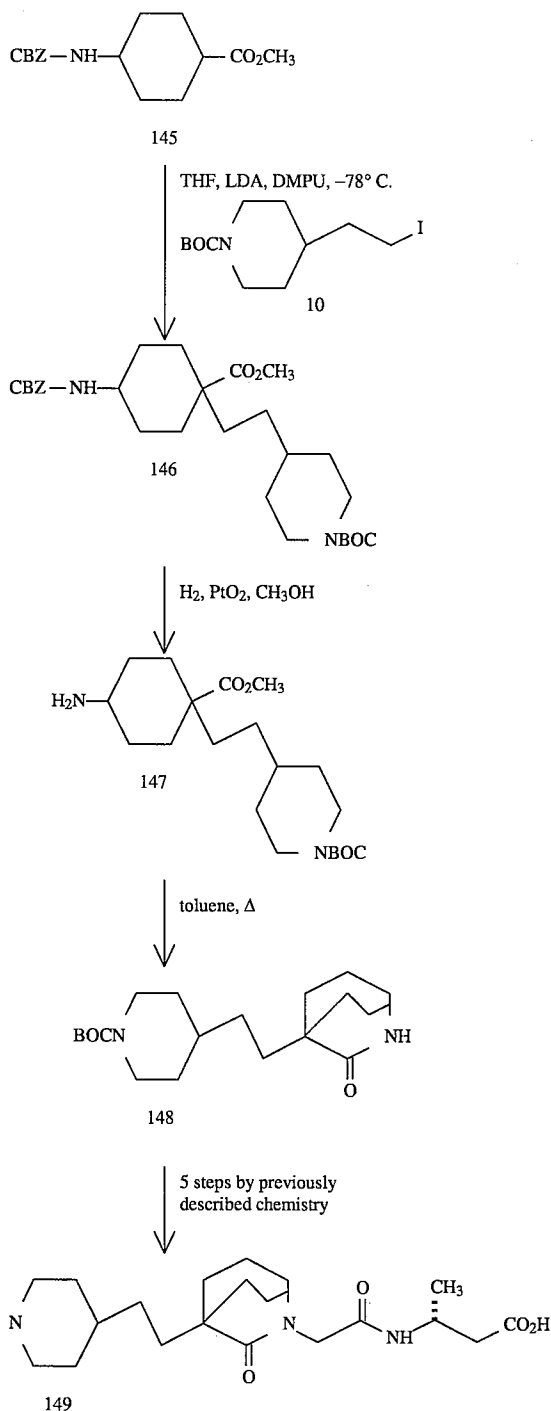
SCHEME 18
