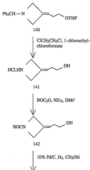
-continued SCHEME 17
