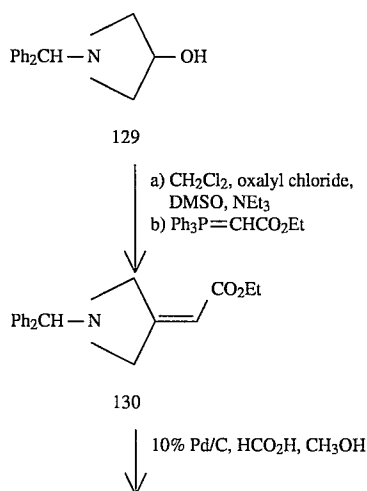
SCHEME 16
