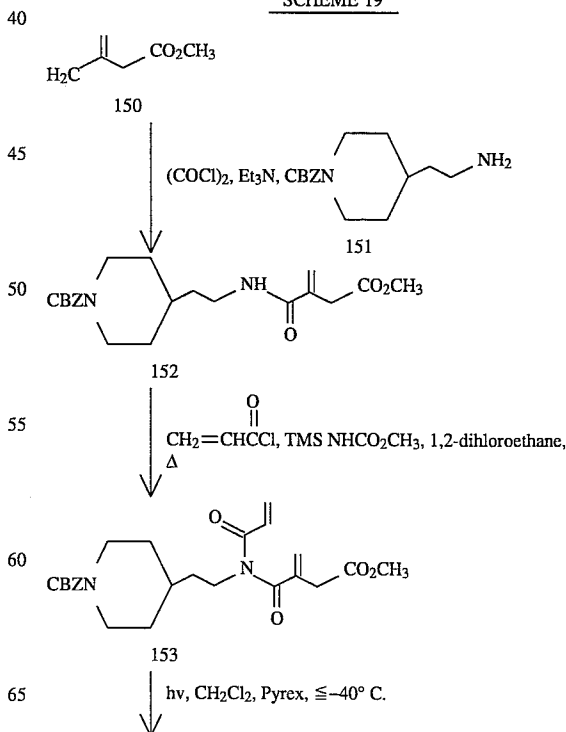
SCHEME 19
