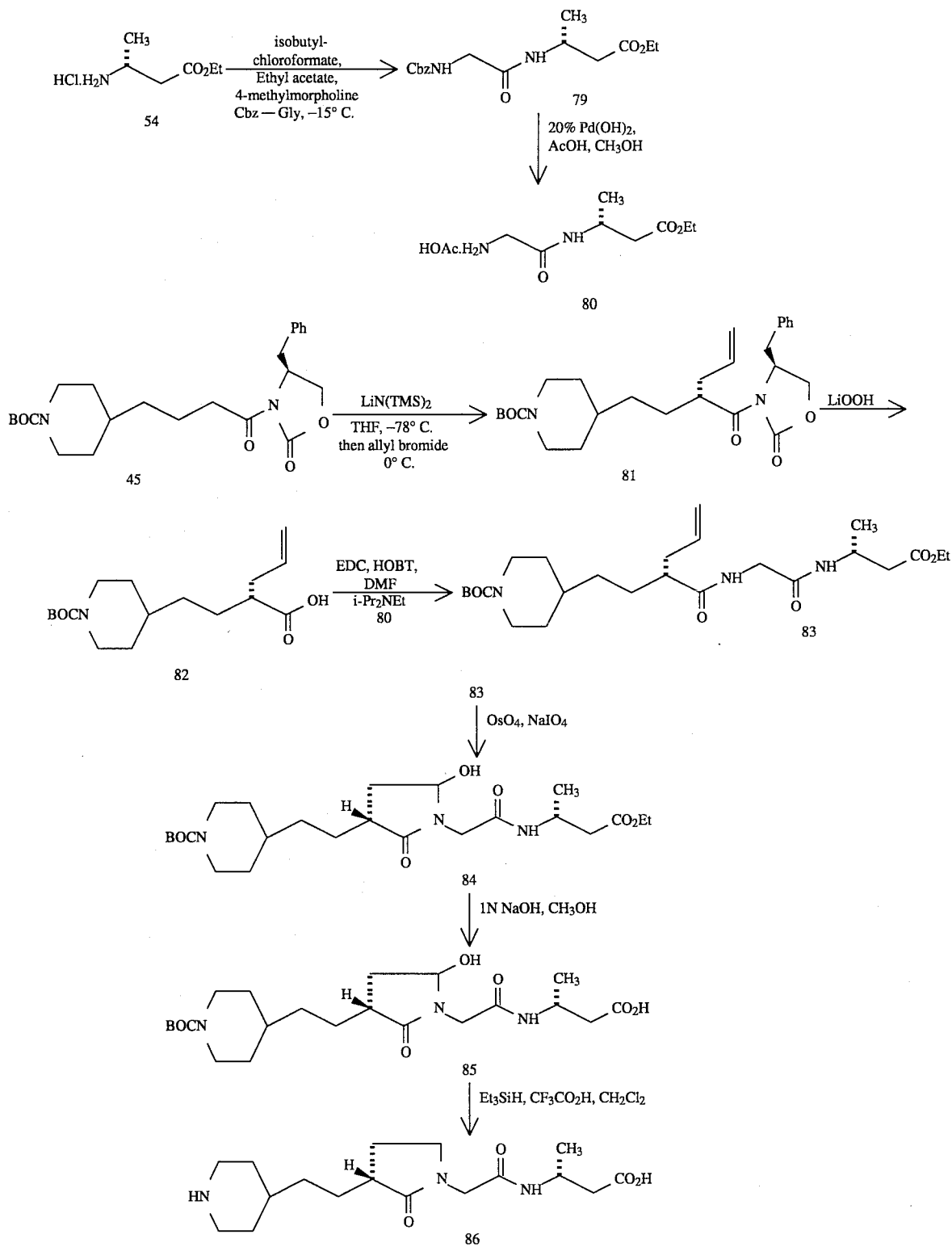
SCHEME 10
