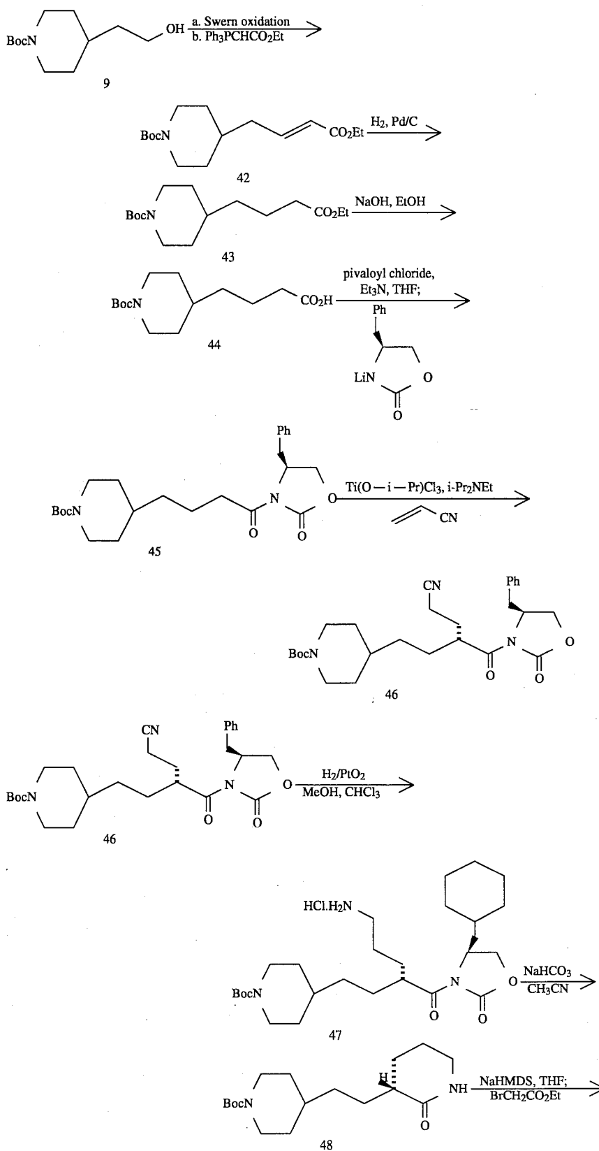
SCHEME 7
