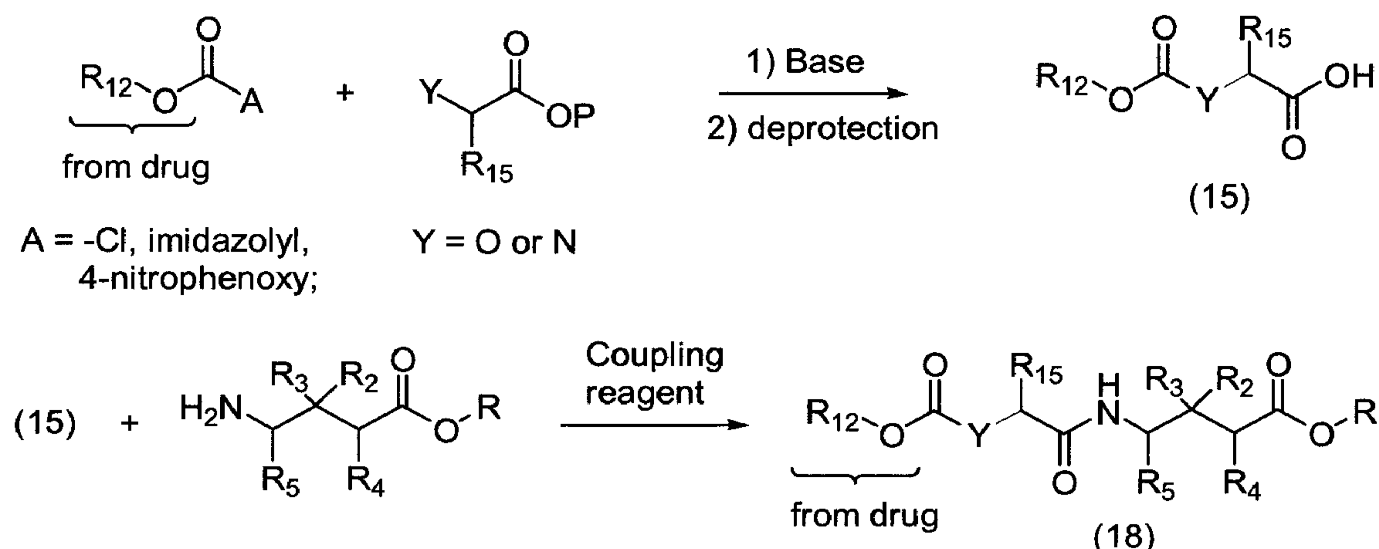
Scheme 7
