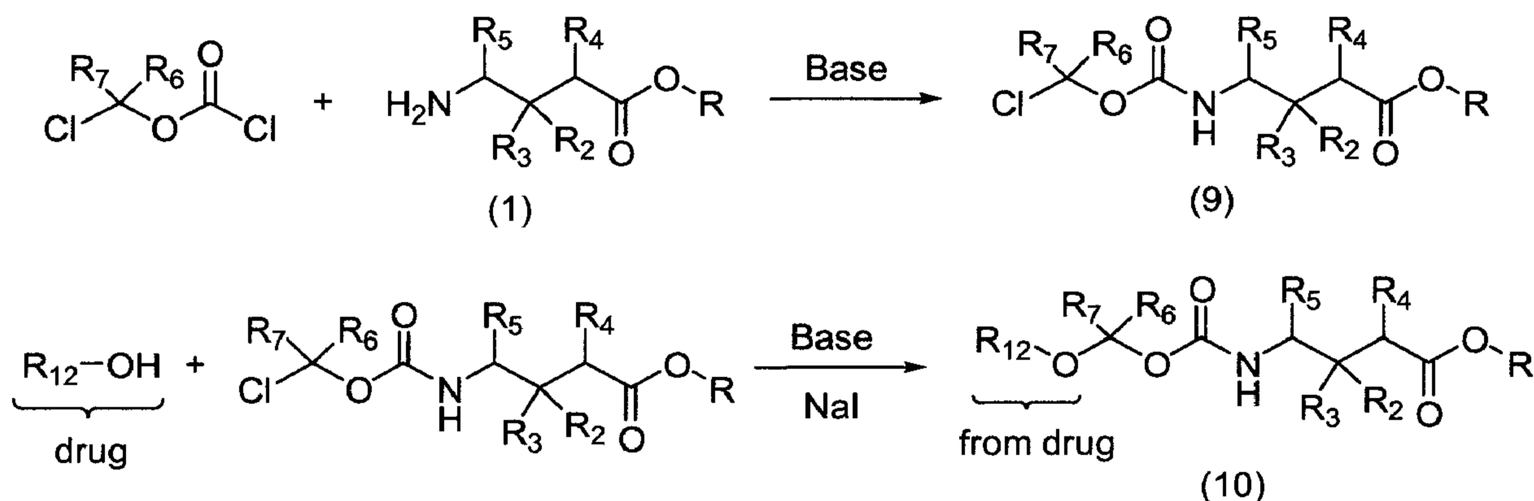
Scheme 4
