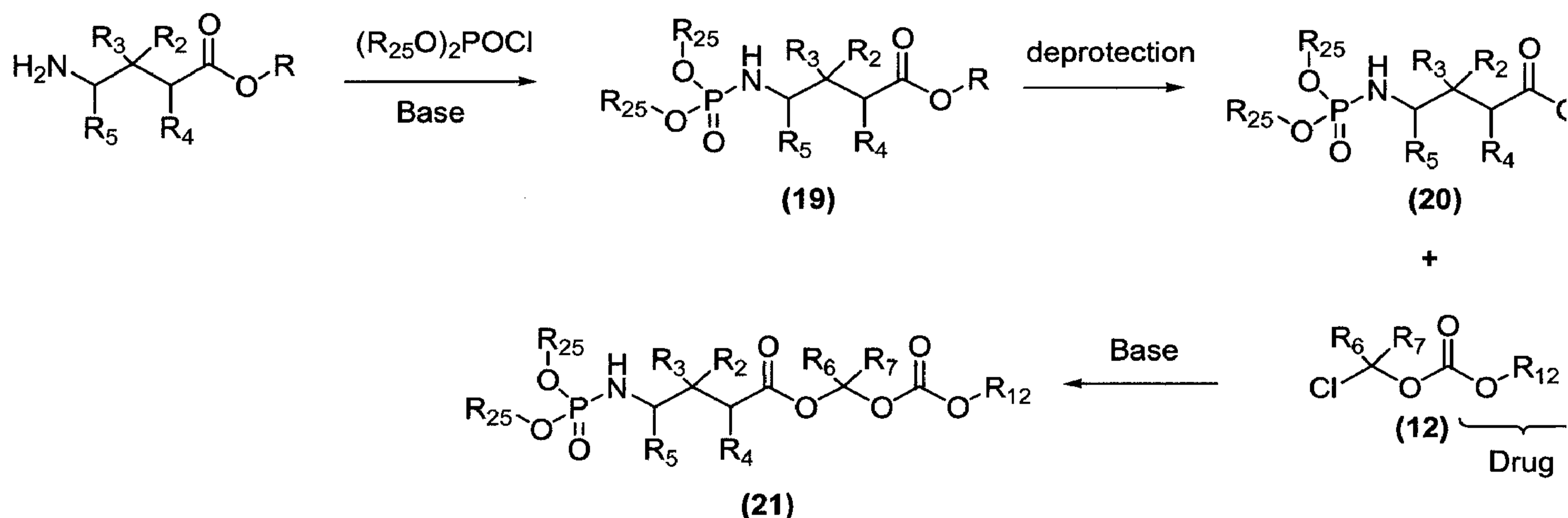
Scheme 8
