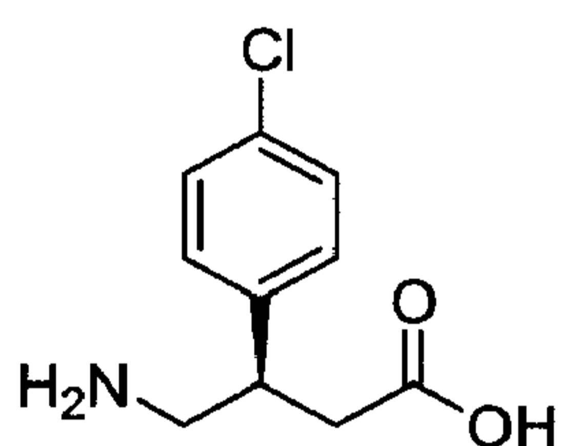
Baclofen-(a)
