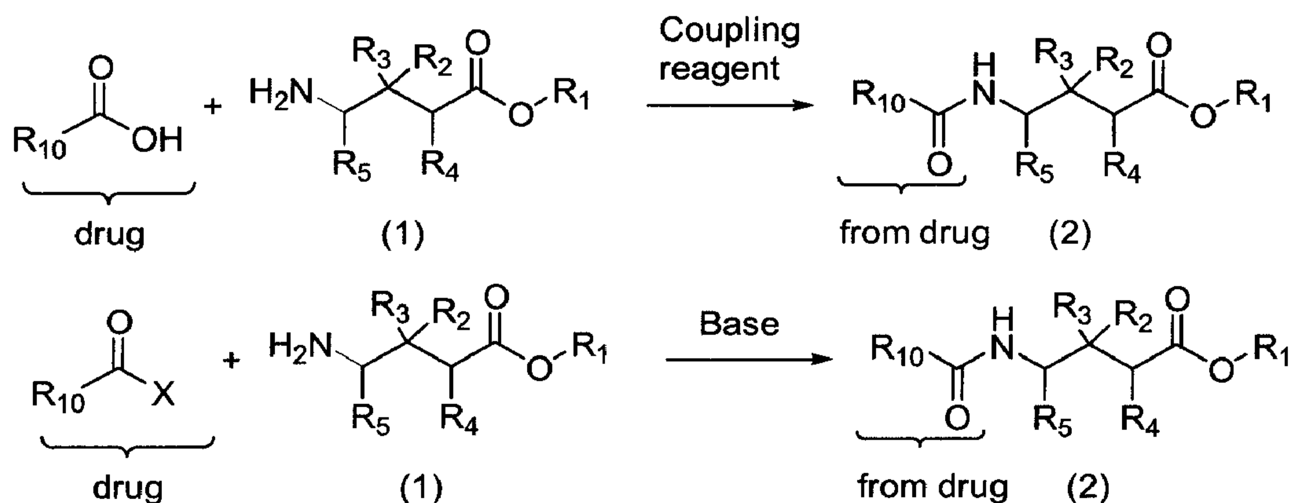
Scheme 1
