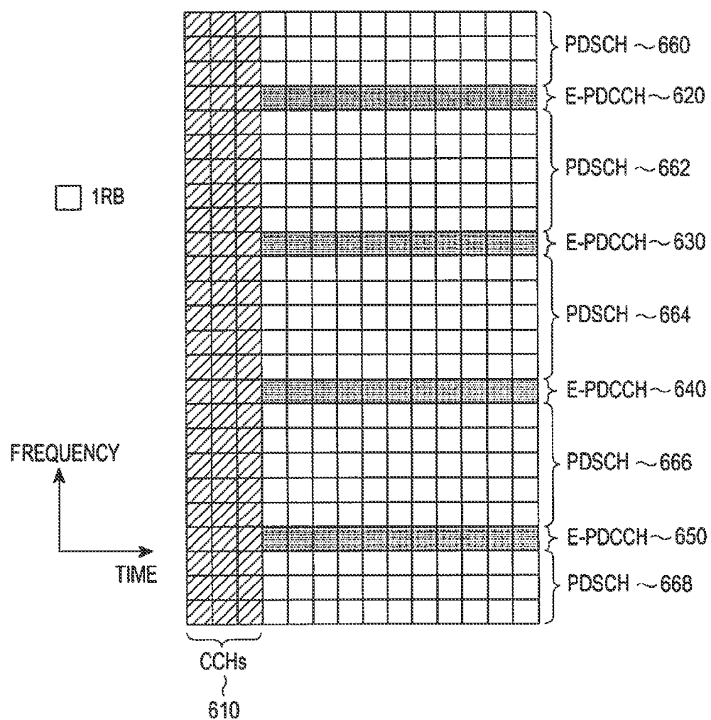
FIG. 6 (PRIOR ART)
