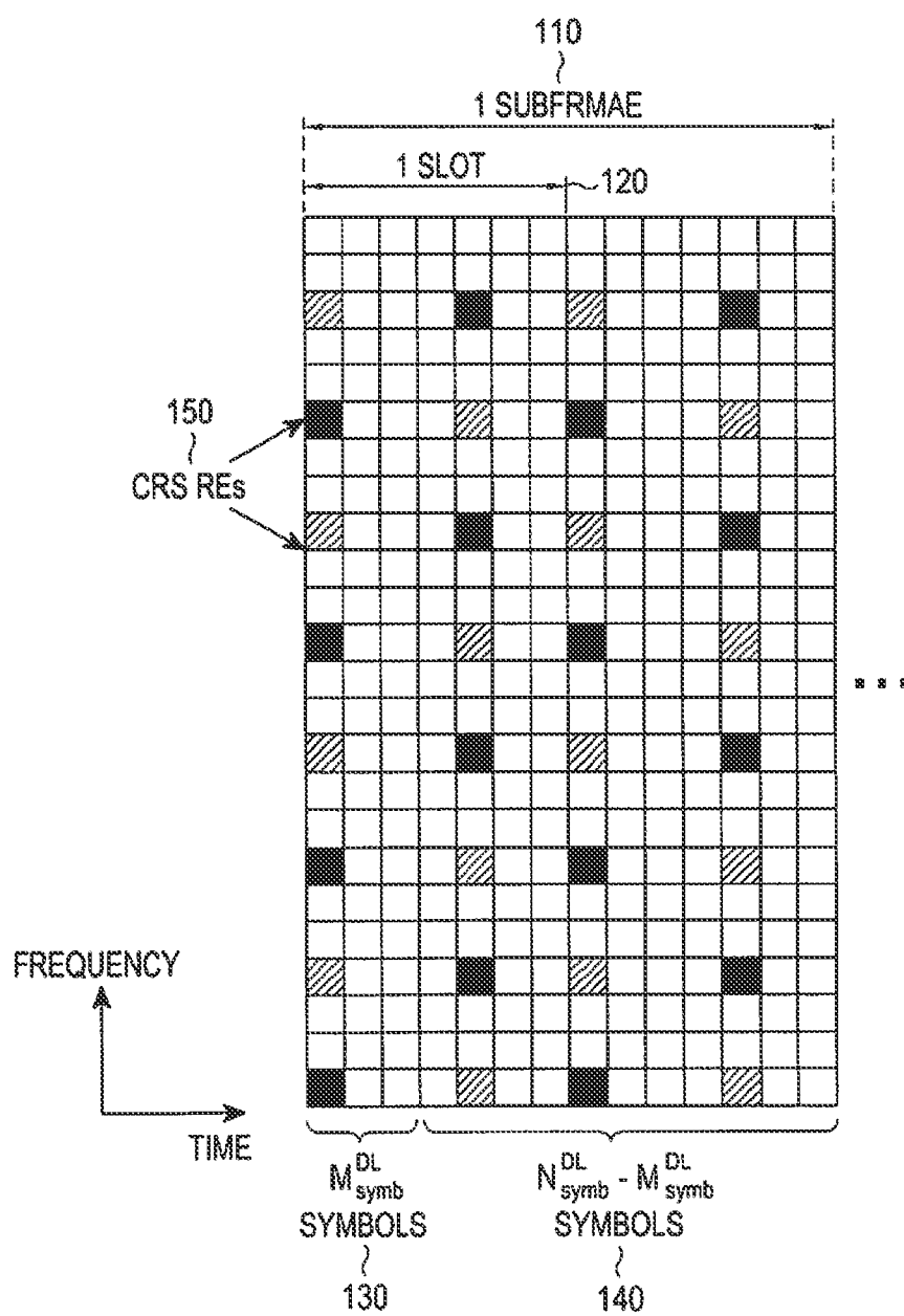
FIG.1 (PRIOR ART)
