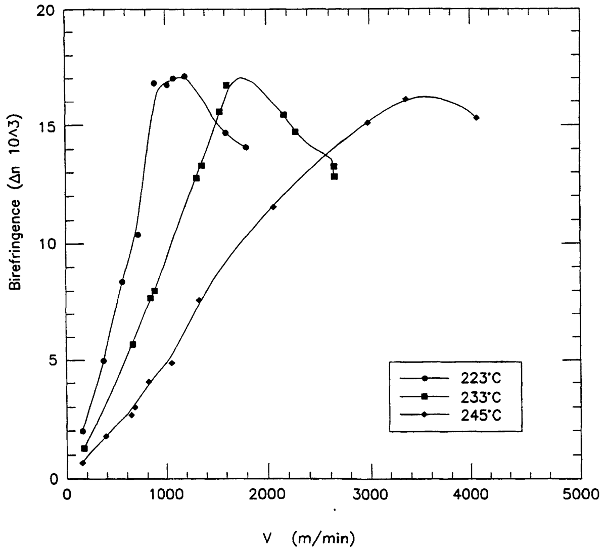
FIG. 12 Fiber birefringence as a function of take-up velocity ( V ) for different melt temperatures (223, 233, and 245°C) and constant melt throughput of 2.95 g/min or 0.74 g/min/hole.
