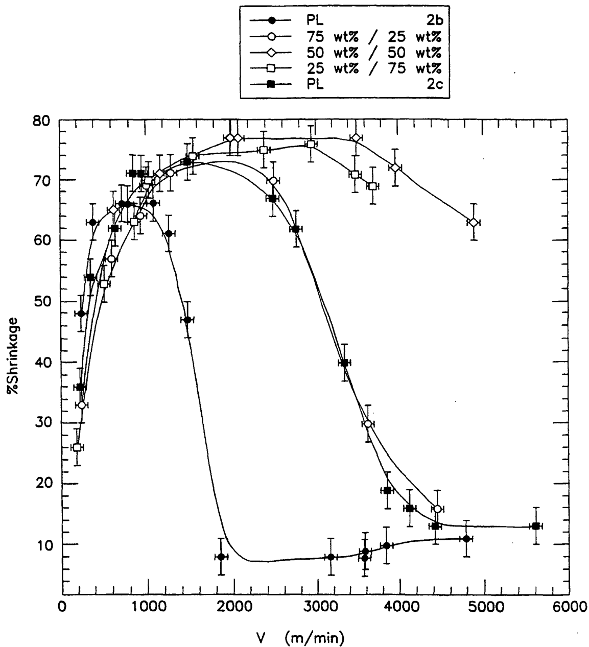
FIG. 22 Fiber shrinkage as a function of take-up velocity ( V ) for two polymers and their blends. Melt temperature is 233^{\circ}\text{C} , and mass throughput is 2.85\text{ g/min} ( 0.71\text{ g/min/hole} ).
