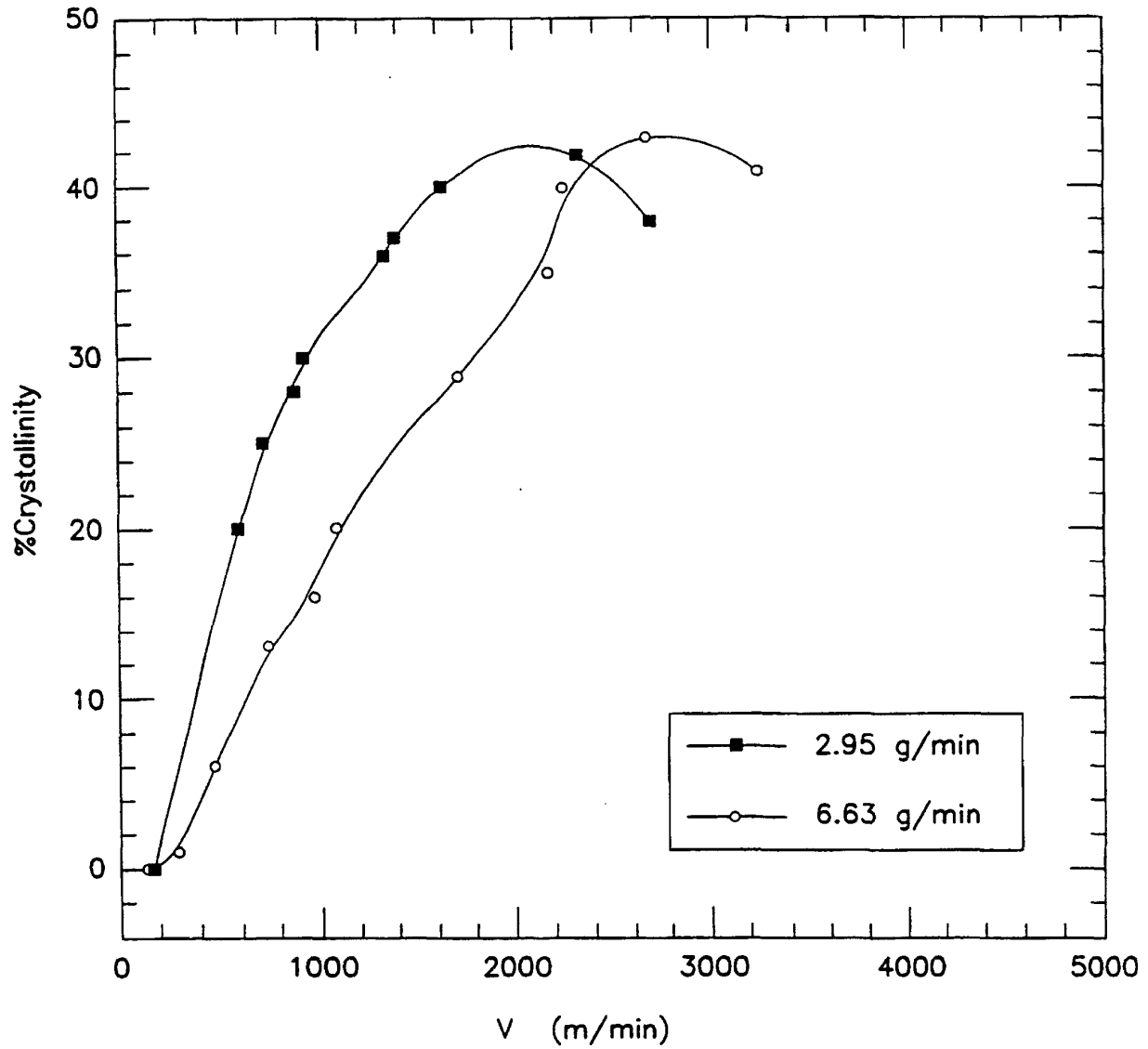
FIG. 14 Amount of crystallinity as a function of take-up velocity ( V ) for different melt throughput (2.95 and 6.63 g/min or 0.74, and 1.66 g/min/hole) and constant melt temperatures of 233°C.
