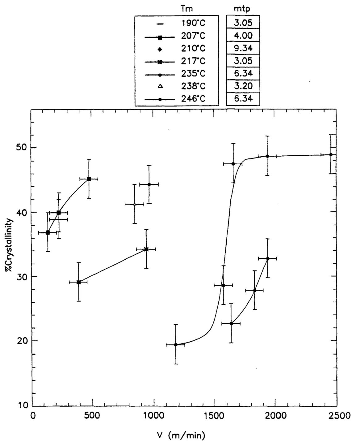
FIG. 8 Amount of crystallinity as a function of take-up velocity ( V ) for different melt temperature ( T_m ) and melt throughput (mtp).
