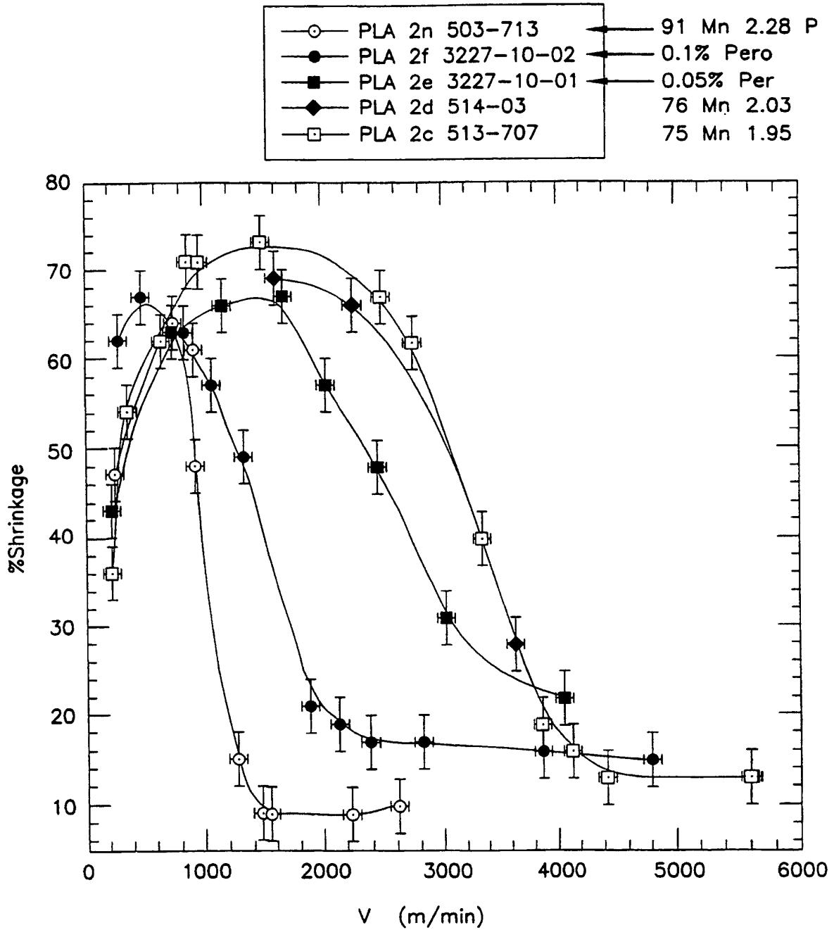
FIG. 18 Shrinkage as a function of take-up velocity (V) for different polymers. Melt temperature is 233°C, and mass throughput is 2.85 g/min (0.71 g/min/hole).
