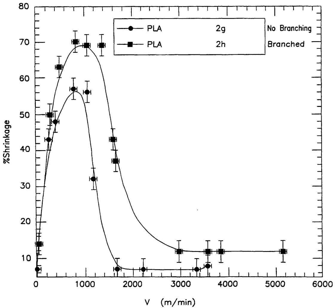
FIG. 20 Effect of branching on %shrinkage. Melt temperature is 233°C, and mass throughput is 2.85 g/min (0.71 g/min/hole).
