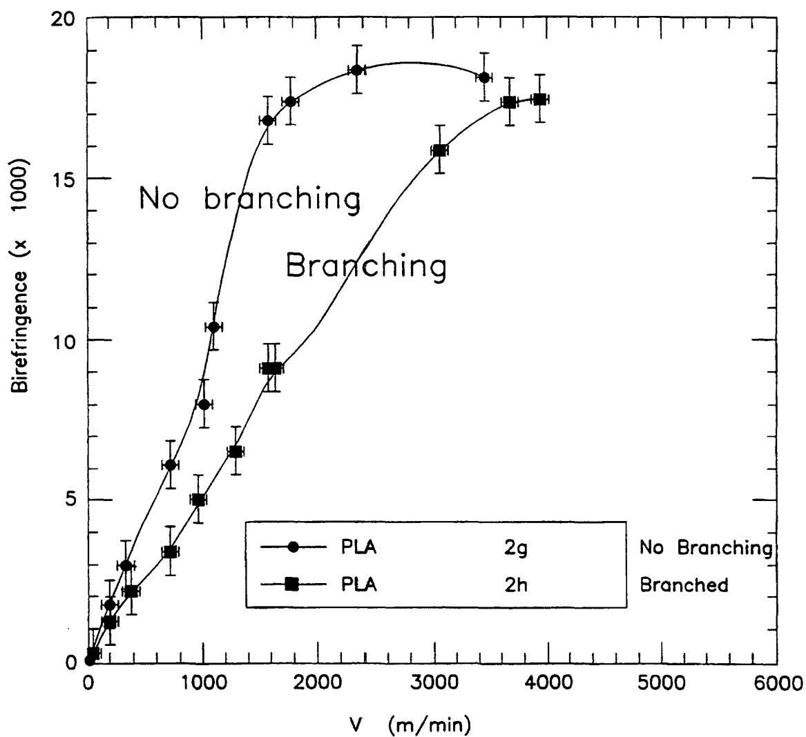
FIG. 19 Effect of branching on fiber birefringence. Melt temperature is 233°C, and mass throughput is 2.85 g/min (0.71 g/min/hole).
