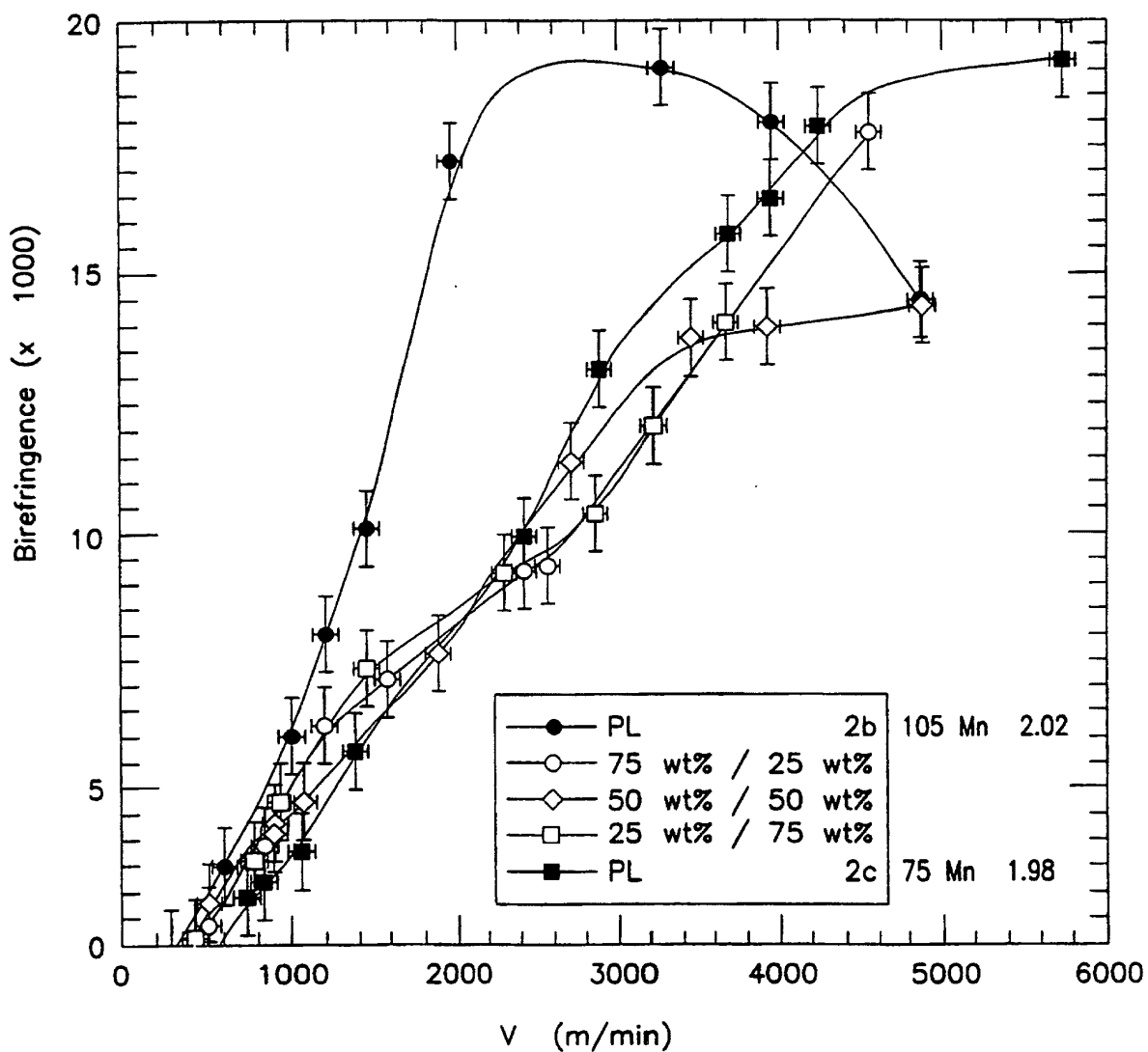
FIG. 21 Fiber birefringence as a function of take-up velocity ( V ) for two polymers and their blends. Melt temperature is 233^{\circ}\text{C} , and mass throughput is 2.85\text{ g/min} ( 0.71\text{ g/min/hole} ).
