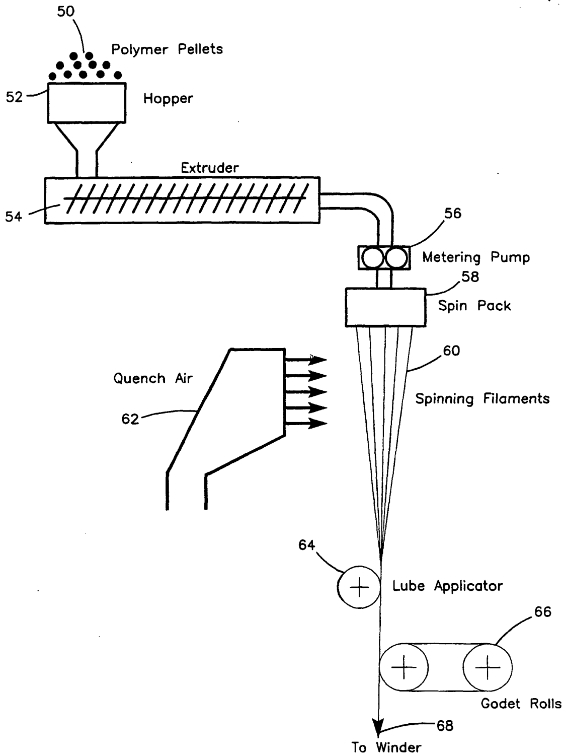
Melt Spinning Process
