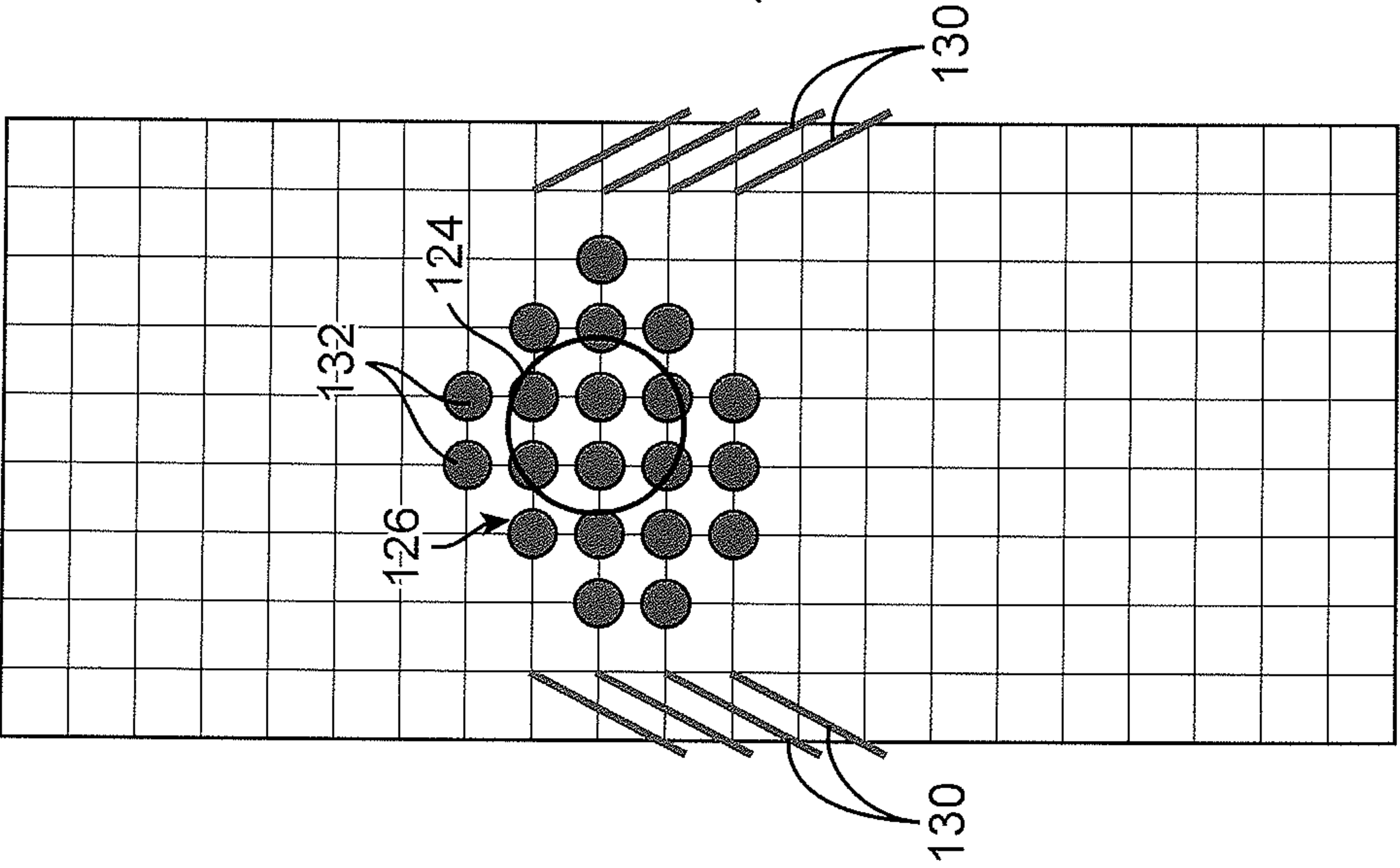
Activated nodes (14 μm fibers)
