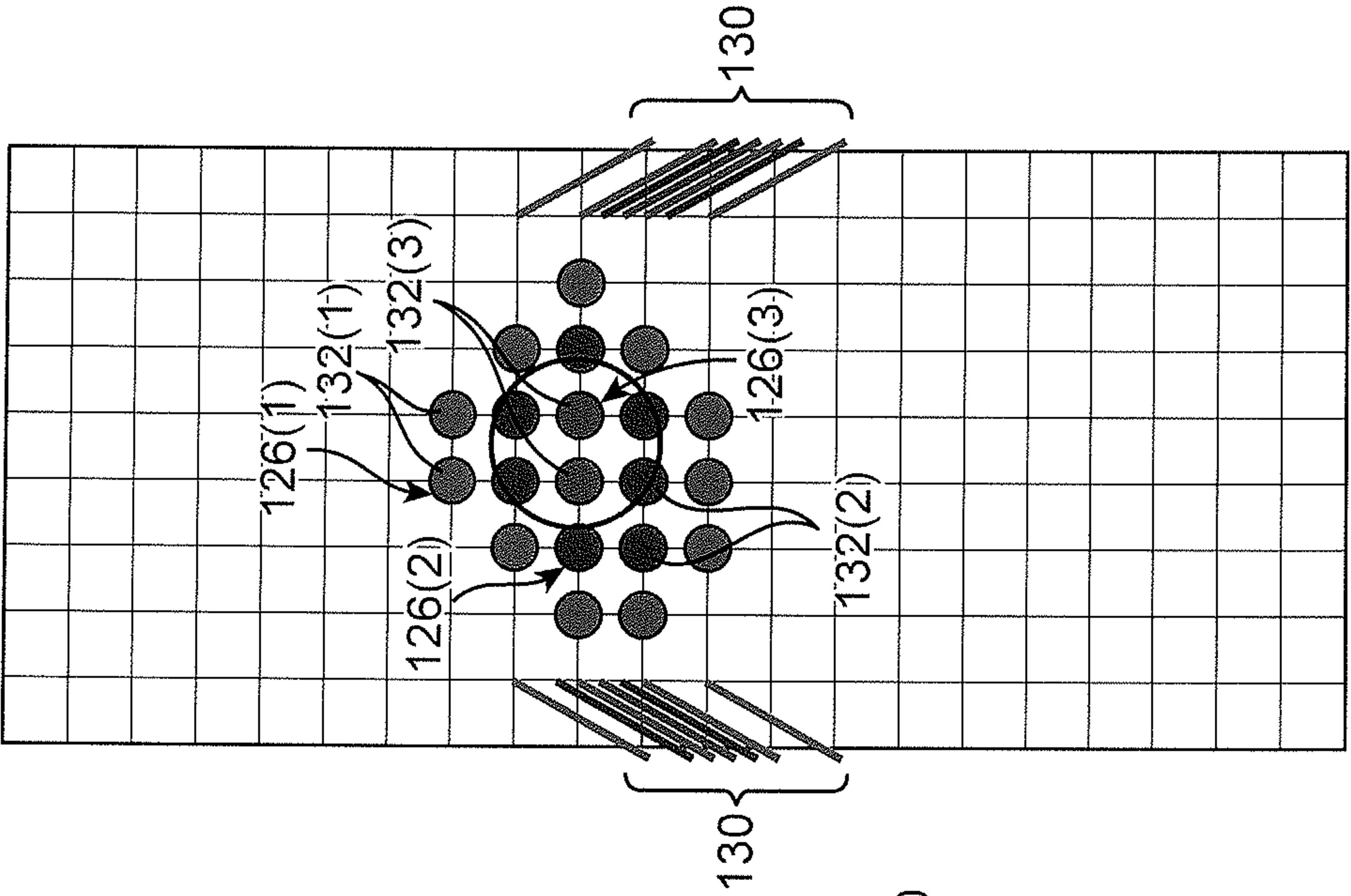
Activated nodes (14, 12 and 11 μm fibers)
