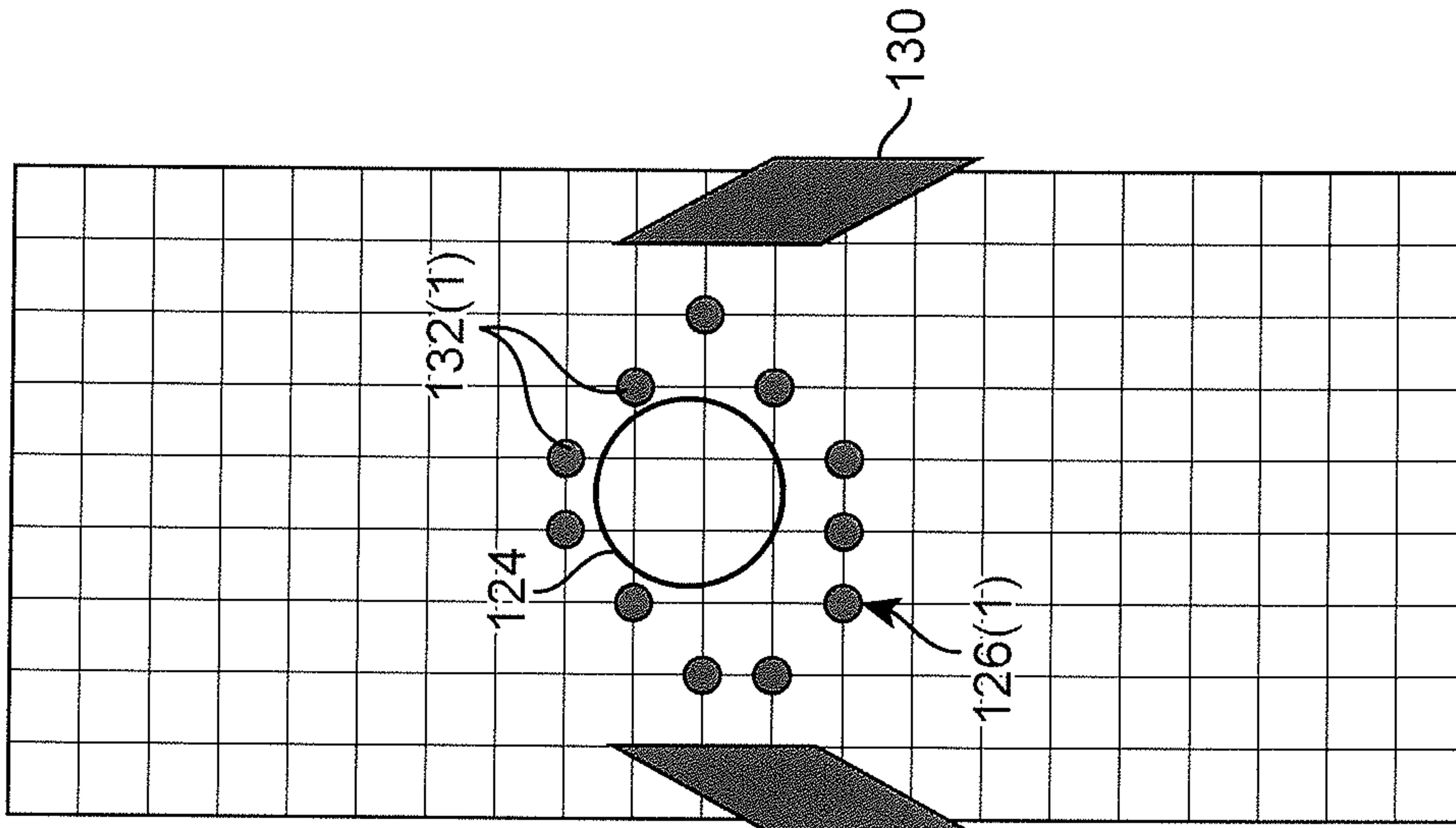
Boundary of activated nodes (14 \mu\text{m} fibers)
