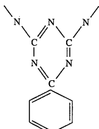
Benzoquanamine
