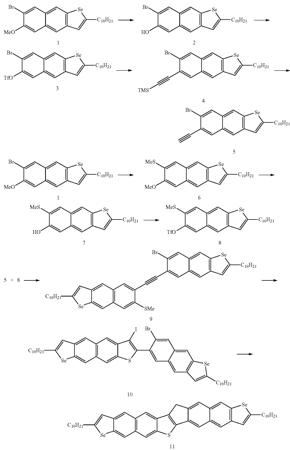
[Reaction Scheme 3]
