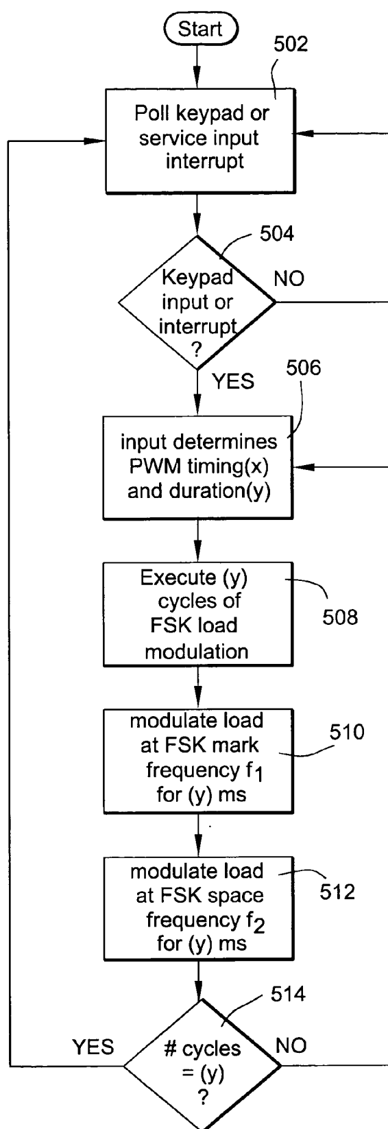
EXAMPLE MODULATED LOAD FLOWCHART
