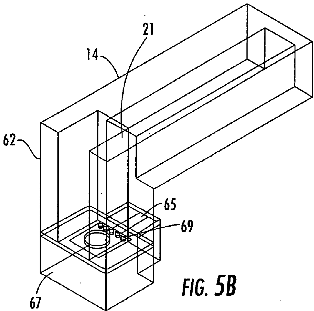
RIDGE WAVEGUIDE BEND AND PROBE DETAILS.
