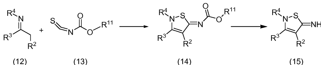
Scheme 5
