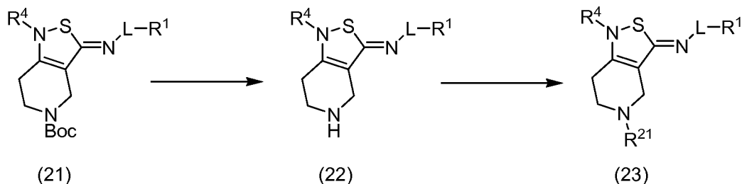
Scheme 8
