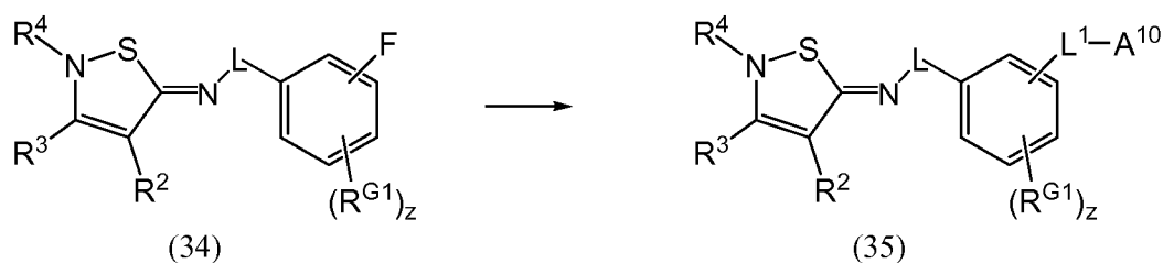
Scheme 14
