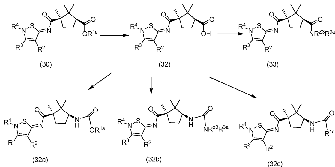
Scheme 13
