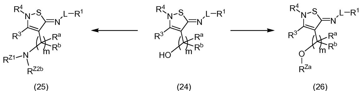
Scheme 9
