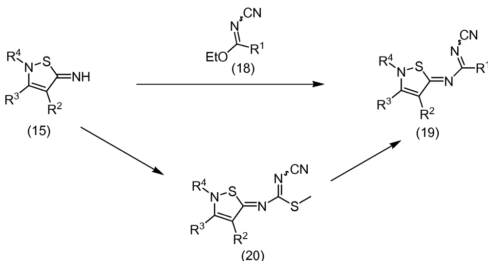
Scheme 7
