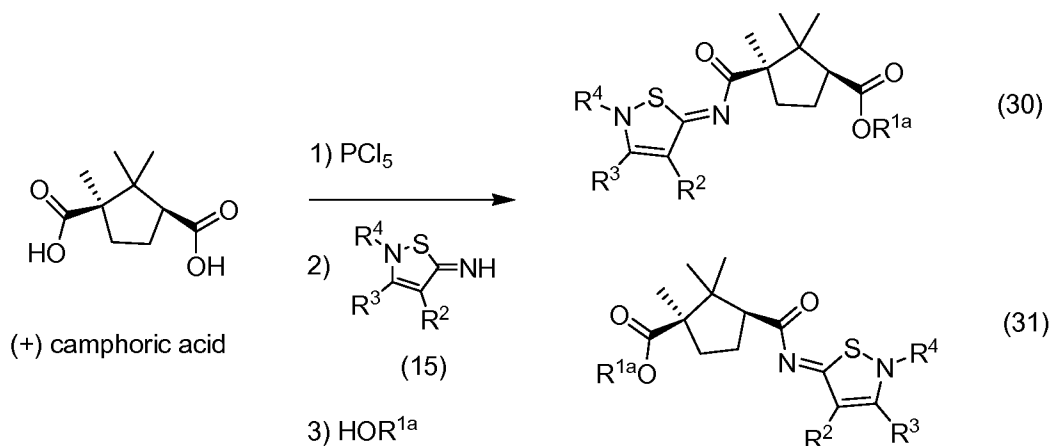
Scheme 12
