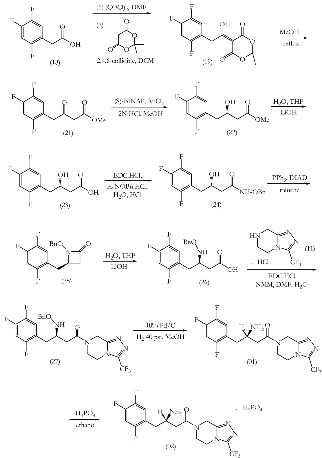
Scheme 4
