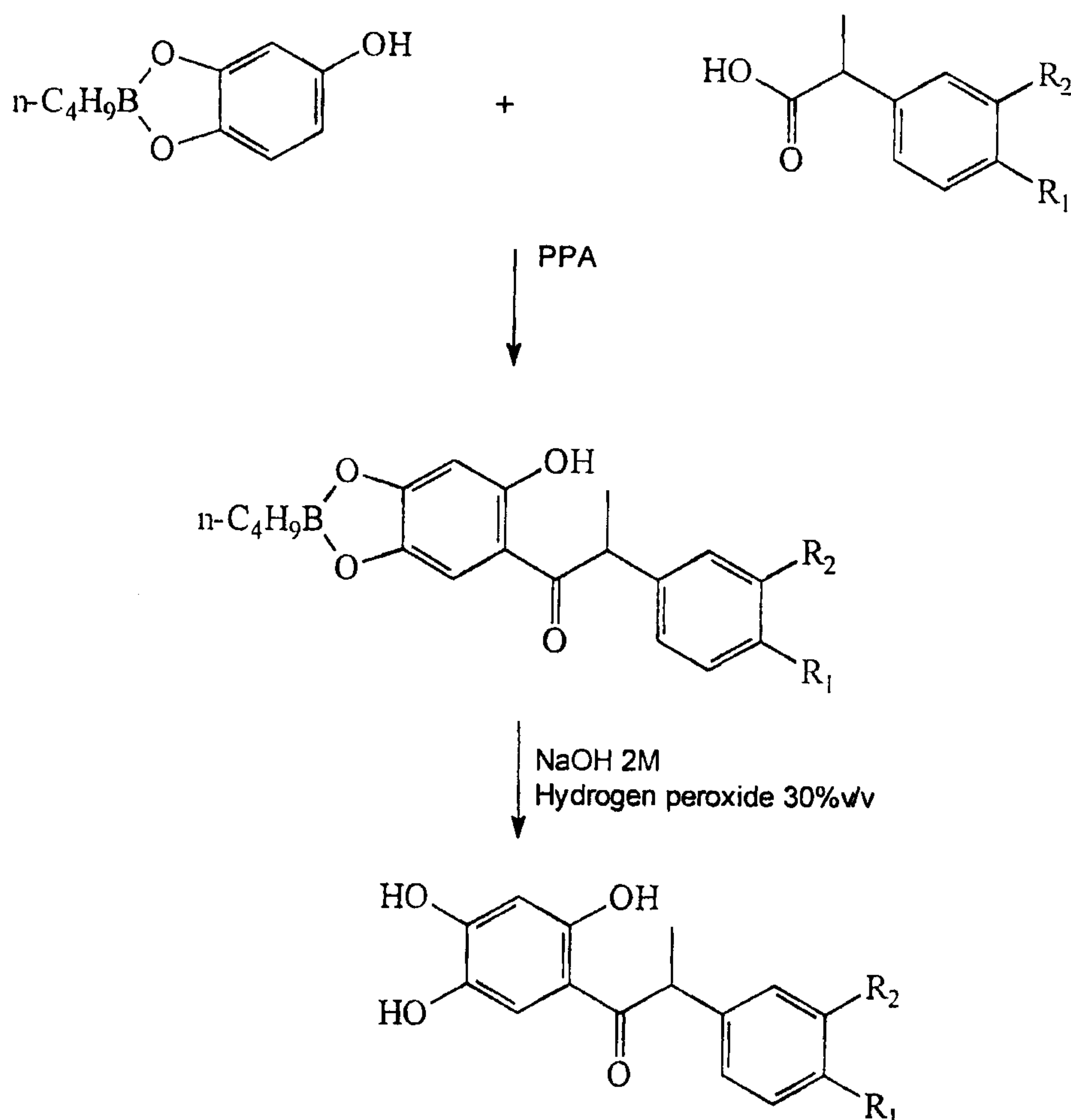
Scheme 3
