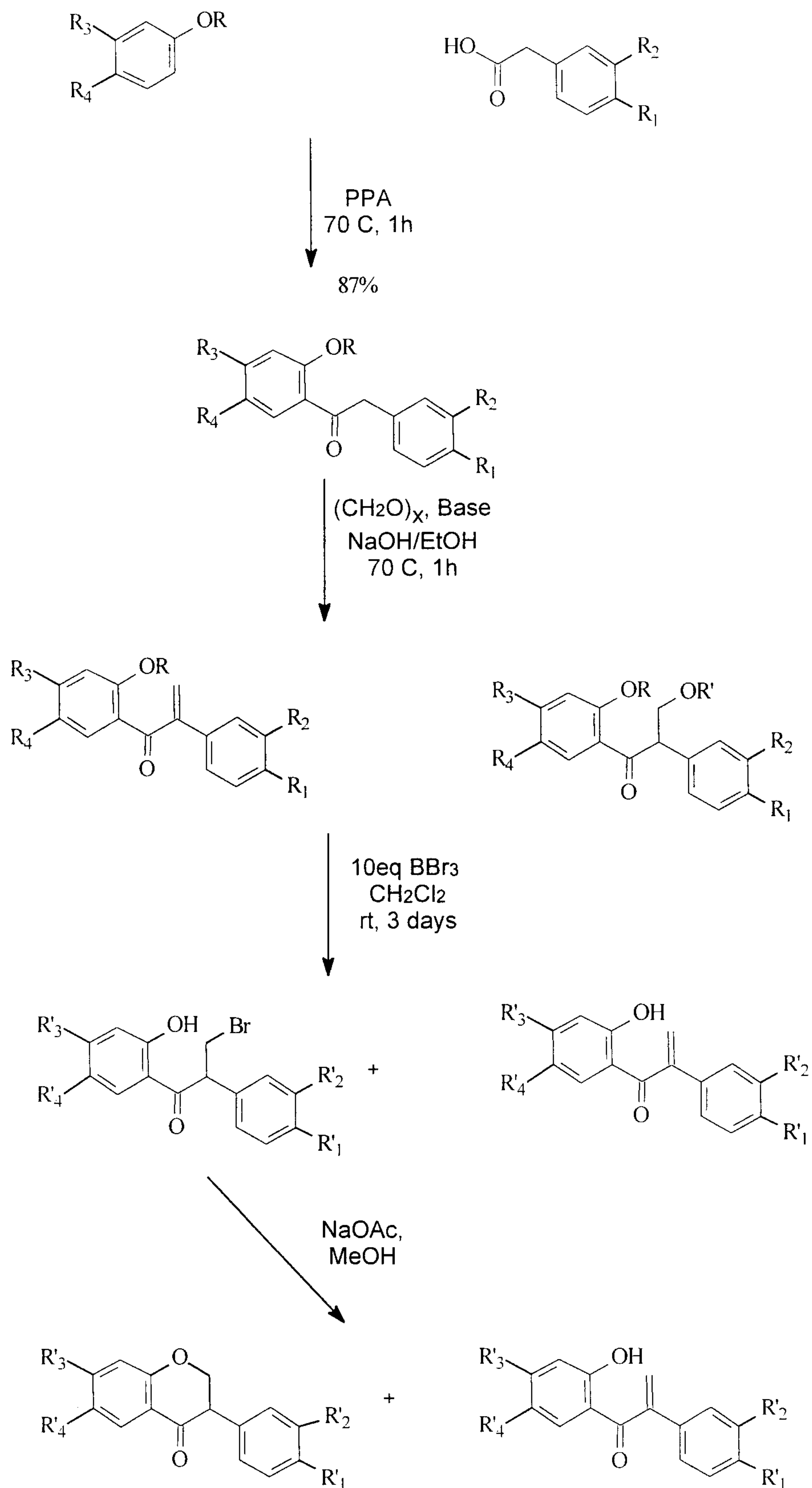
Scheme 7
