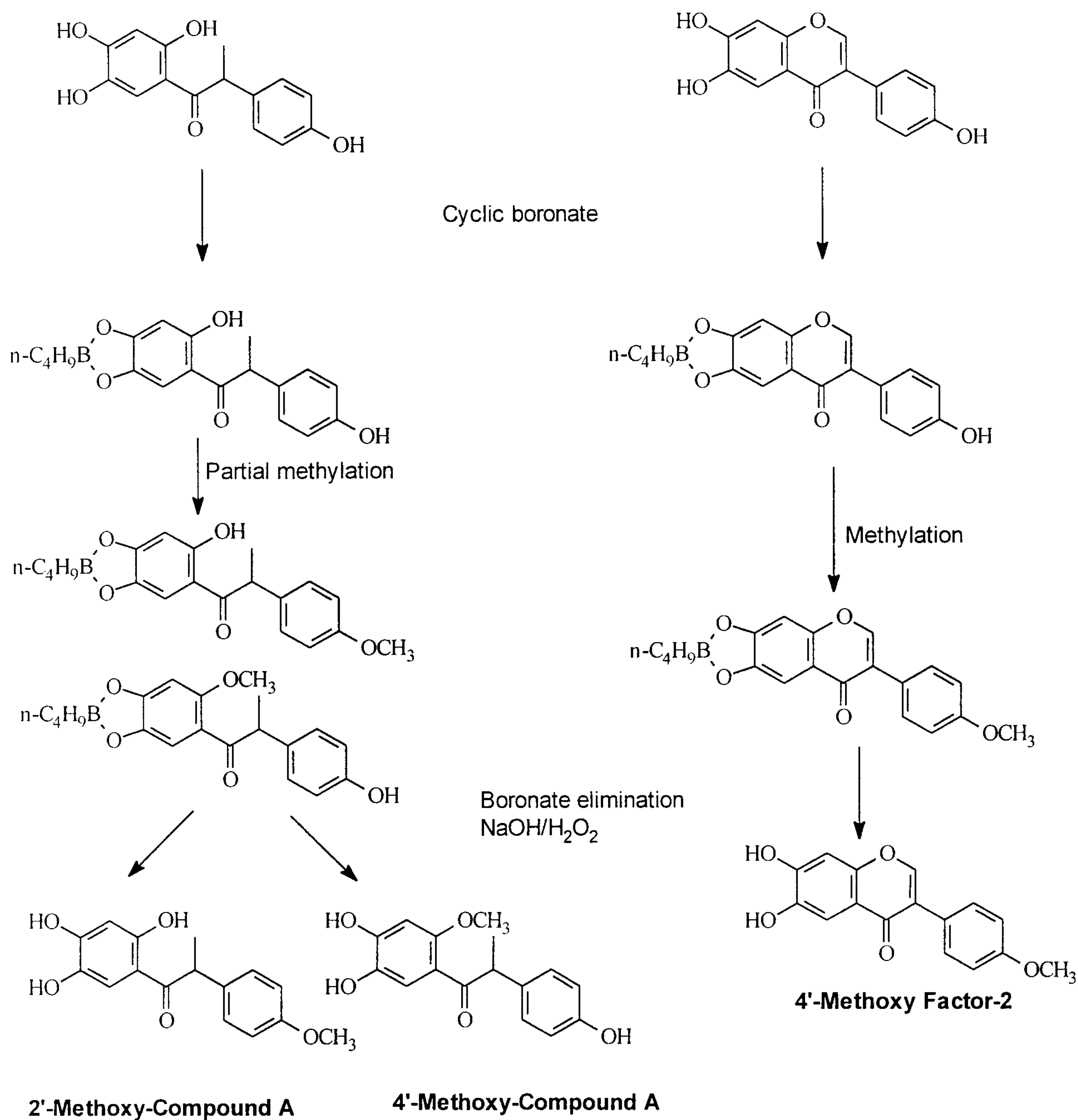
Scheme 4B
