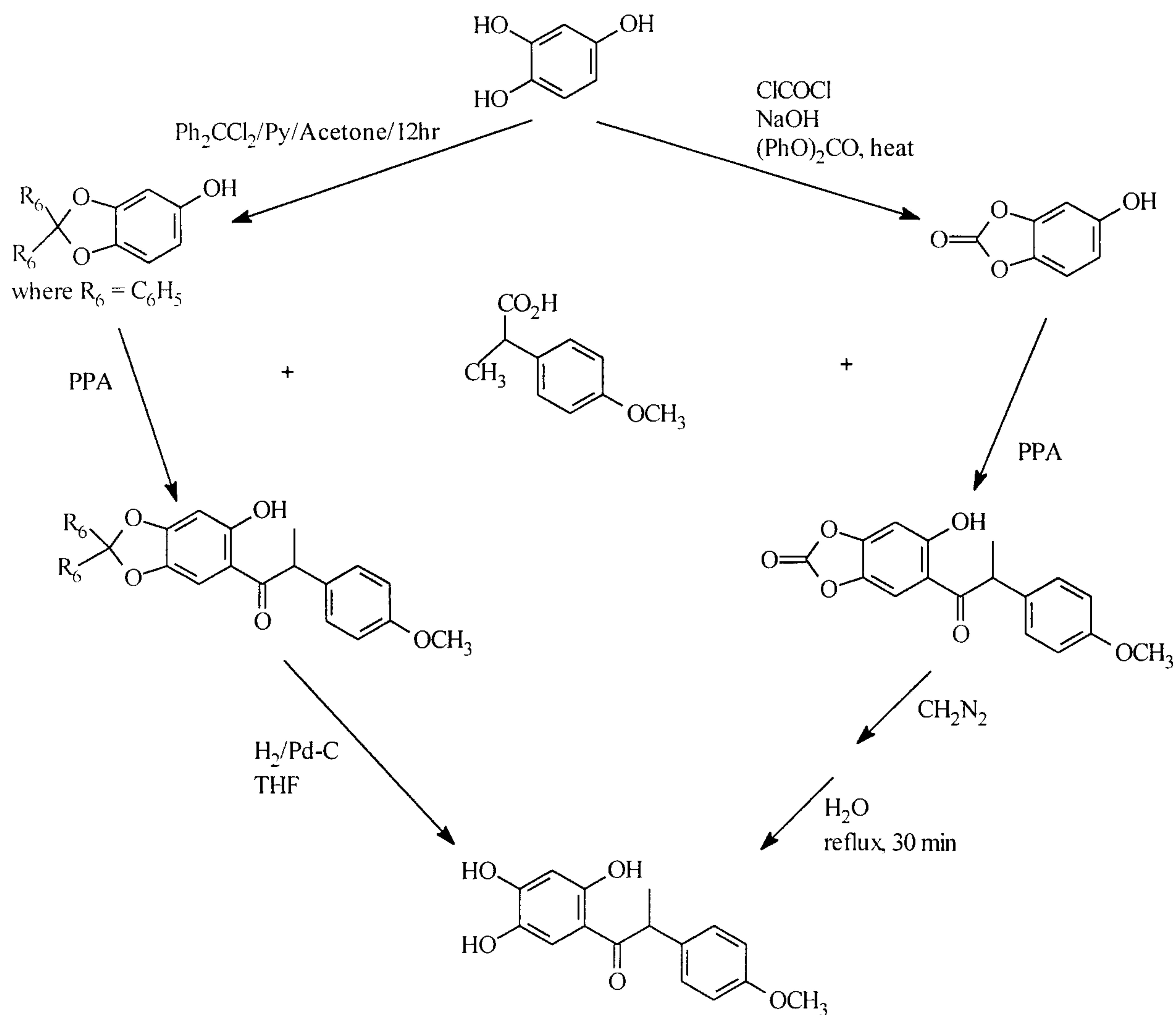
Scheme 4A
